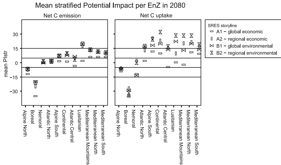
Fig. 12 Scatter plots of stratified potential impacts (PIstr) for the indicators relevant for the climate regulation sector: net carbon emission and uptake. Note that values for net carbon emission were multiplied by -1 , therefore all positive values correspond to positive change and vice versa
