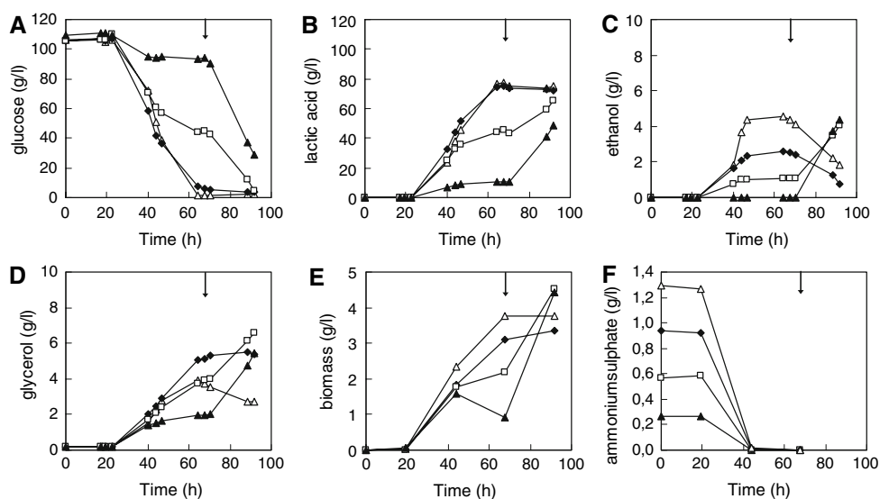
Fig. 2 Conversion of glucose by R. oryzae CBS 112.07 to lactic acid (b), ethanol (c), glycerol (d) and fungal biomass (e) with initial C/N ratio of 603/1 [0.31 g/l (\text{NH}_4)_2\text{SO}_4 ] (dark filled triangle), 302/1 [0.63 g/l (\text{NH}_4)_2\text{SO}_4 ] (open square), 201/1 [0.94 g/l (\text{NH}_4)_2\text{SO}_4 ] (dark filled diamond) and 151/1 [1.25 g/l (\text{NH}_4)_2\text{SO}_4 ] (open triangle). Figure f represents the (\text{NH}_4)_2\text{SO}_4 concentration in the fermentation medium. The arrow represents the moment of addition of ammonium sulphate
