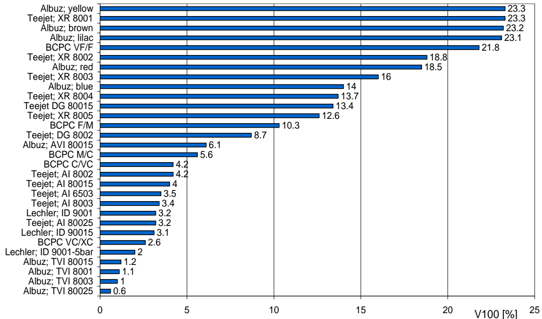
Figure 2. Ranking of measured nozzles used in orchard spraying based on volume of drops smaller than 100 \mu\text{m} ( V_{100} )
