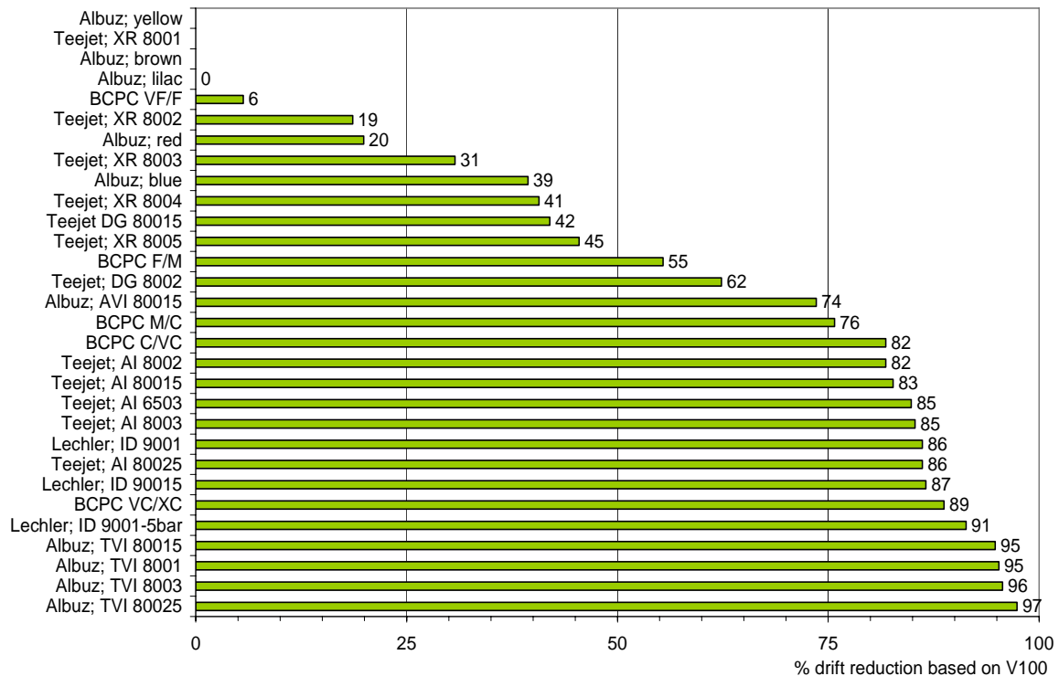
Figure 3. Potential in spray drift reduction based on V_{100} ( DR_{V100} ) relative to the reference nozzle Albus Lilac (7 bar spray pressure)
