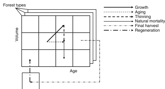
Fig. 1 Structure and simplified processes of the matrix model EFISCEN v3.2
