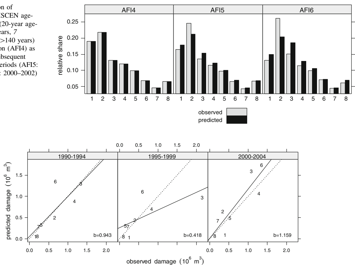
Fig. 5 Observed versus predicted 5-year Ips typographus damages for Austria's federal provinces (1 Burgenland, 2 Kärnten–Carinthia, 3 Niederösterreich–Lower Austria, 4 Oberösterreich–Upper Austria, 5 Salzburg, 6 Steiermark–Styria, 7 Tirol–Tyrol, 8 Vorarlberg) in three
