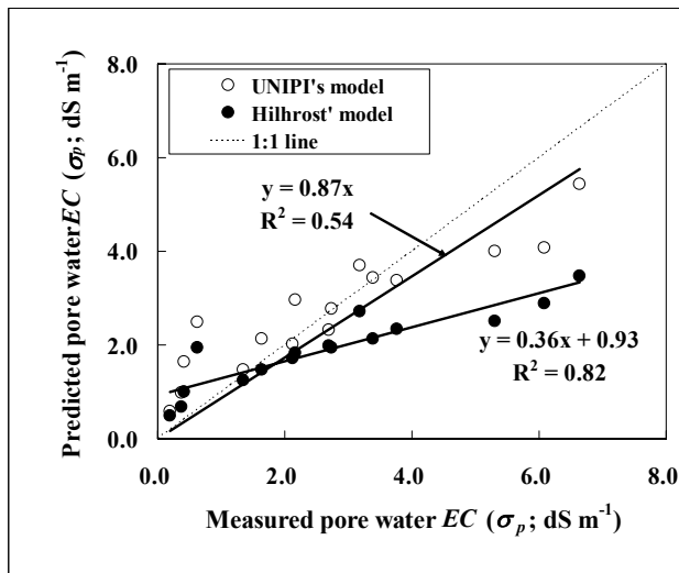
Fig. 6. The relationship between measured and predicted values of pore water EC ( \sigma_p ) in a peat-pumice mixture irrigated to container water capacity with nutrient solution of different salinity (EC) and then dried in air to desired volumetric water content ( \theta ). The EC was measured in the water collected by centrifugation or calculated from the bulk EC ( \epsilon ) provided by WET ® sensor using two different equations (see text for details).
