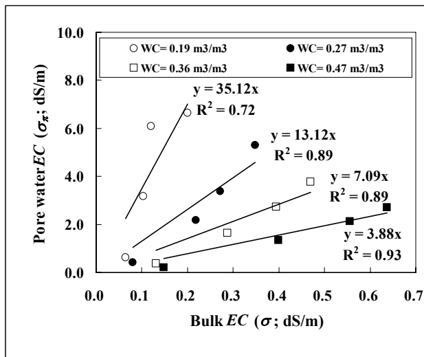
Fig. 5. The relationship between bulk EC ( \sigma , as measured by means of WET ® sensor) and pore water EC ( \sigma_p ) in a peat-pumice mixture irrigated to container water capacity with nutrient solutions of different salinity (EC; the values are reported in the box) and then dried in air to desired water content (WC).
