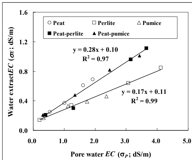
Fig. 2. The relationship between pore water EC ( \sigma_p ) and water extract EC ( \sigma_e ) for different horticultural substrates. Pore water was collected by means of centrifugation, whereas water extract was obtained by means of 1 substrate: 2 water suspension method.
