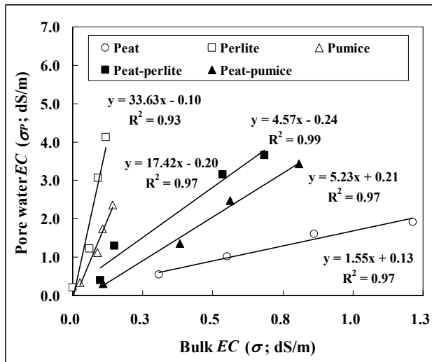
Fig. 3. The relationship between bulk EC ( \sigma , as measured by means of WET ® sensor) and pore water EC ( \sigma_p ) in different horticultural substrates.
