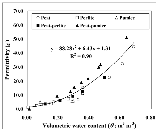
Fig. 1. The relationship between permittivity ( \epsilon , as measured by means of WET ® sensor) and volumetric water content ( \theta ) in different horticultural substrates.
