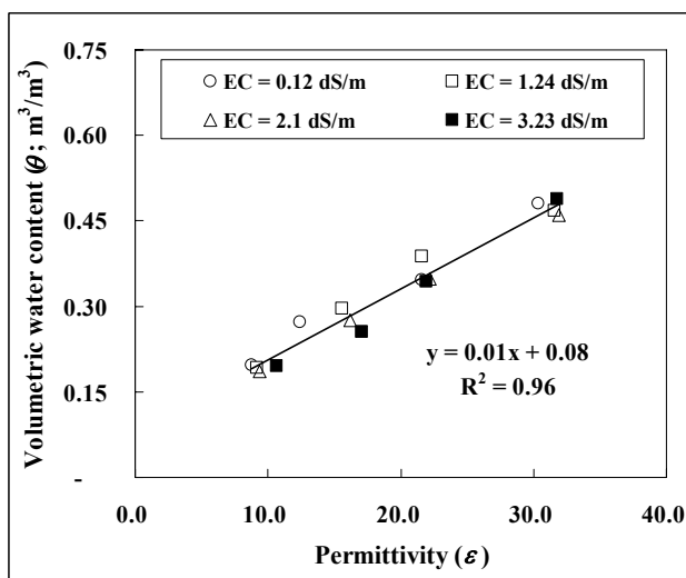
Fig. 4. The relationship between permittivity ( \epsilon , as measured by means of WET ® sensor) and volumetric water content ( \theta ) in a peat-pumice mixture irrigated to container water capacity with nutrient solutions of different salinity (EC; the values are reported in the box).
