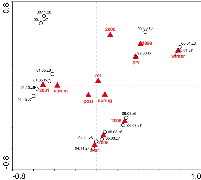
Figure 12. RDA ordination diagram for the dam construction restoration measure with the restoration phase ( pre , post , ref ), year and season variable groups included. The triangles represent the relative effect of the variables; the open circles represent each sample site. Sample sites are labelled by sample year and season and location.
