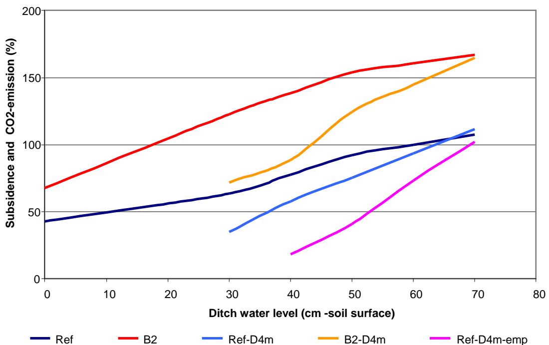
Figure 6 Effect of water management and climate change on subsidence and CO 2 emission of a representative Dutch peatsoil without a thin (< 40 cm) clay layer and a ditch water level of 60 cm below surface. The climatic reference period is 1971 -2000. The considered climate change period is 2071 – 2100 and the IPCC scenario B2 is considered (moderate change). Ref = Reference; B2 = B2 scenario IPCC; Ref-D4m = Reference with submerged drains at 4 m distances; B2-D4m = B2 scenario with submerged drains at 4 m distances; Ref-D4m-emp = Reference with submerged drains at 4 m distances, however, subsidence calculated with empirical relations between ground water level and subsidence (Van den Akker et al., 2007).
