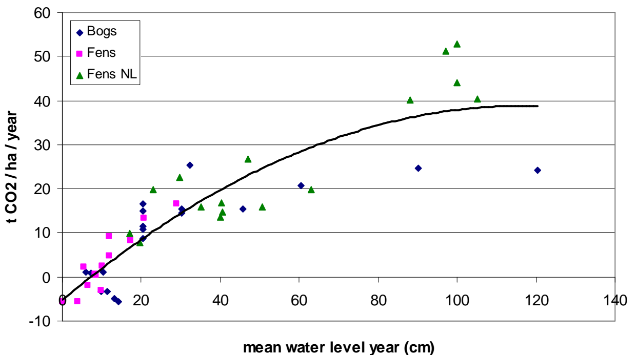
Figure 5 CO 2 emission of peat soils. Agricultural peat soils have at least a mean ditchwater level of 20 cm minus soil surface. Data collected by Couwenberg et al., (2008) based on direct measurements of CO 2 emissions and emissions calculated from measured mean annual subsidence and Van den Akker (Fens NL, unpublished data) based on CO 2 emissions calculated from measured mean annual subsidence.
