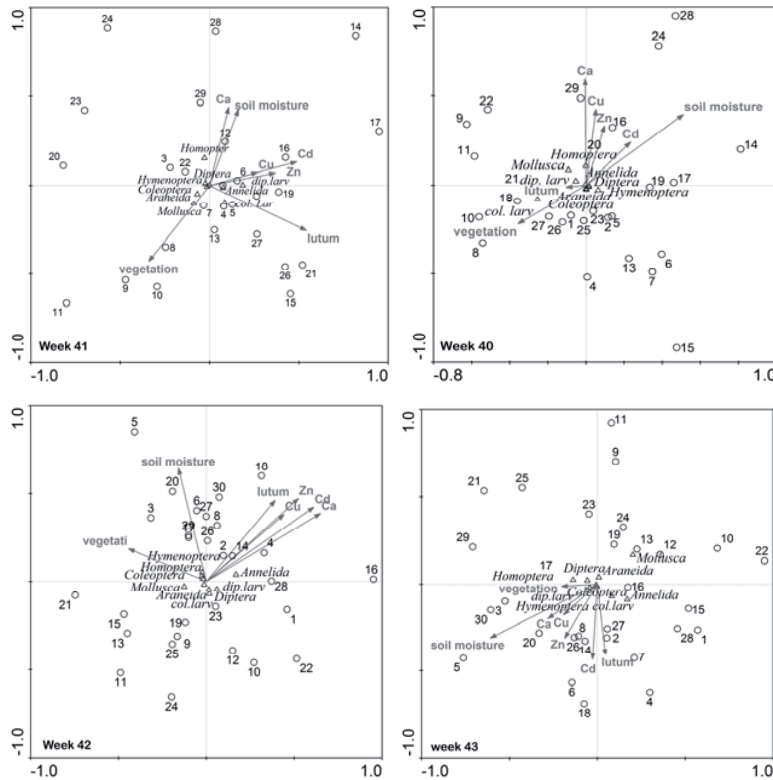
Figure 7. Canonical correspondence analysis of the 30 location in the field on environmental data and taxa variables for the 4 weeks sampled. Abbreviations used: Ca, calcium; col.larv Coleoptera larvae; Cu, copper; dip.larv, Diptera larvae. Metal concentrations are total concentrations (mg/kg DW).
