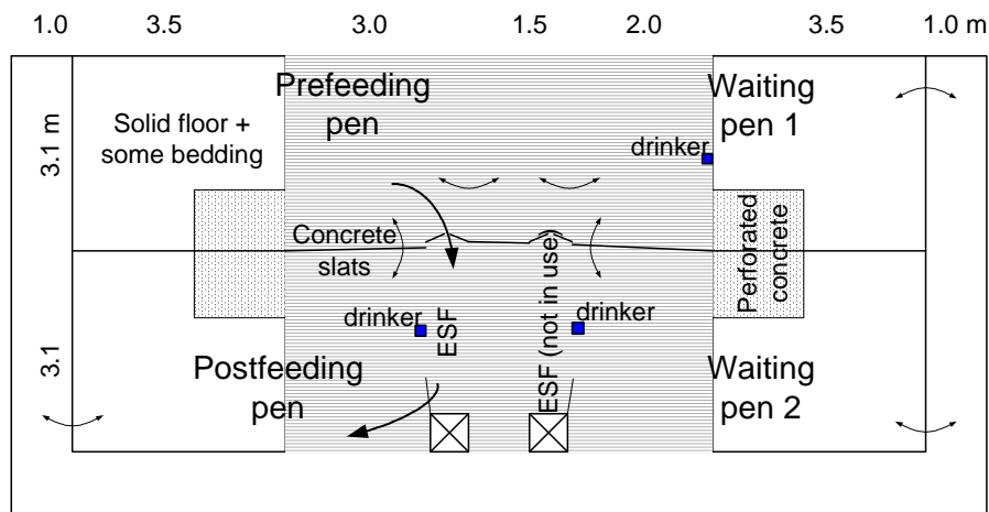
Fig. 1. Layout of the experimental pen; a group of 4 gilts started in the prefeeding pen and passed the ESF one by one to the postfeeding pen; meanwhile the other two groups were waiting in the pens on the right side of the room.
