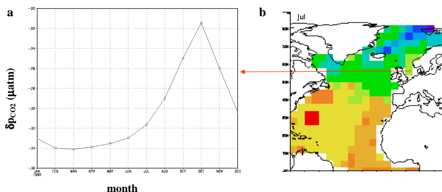
Fig. 5. (a) Monthly dynamics of \delta p_{\text{CO}_2} ( \mu\text{atm} ; 1 atm=1.01325 Pa) as a time series for a pixel in the North Sea (left panel), (b) Spatial representation of \delta p_{\text{CO}_2} for the Atlantic Ocean.
