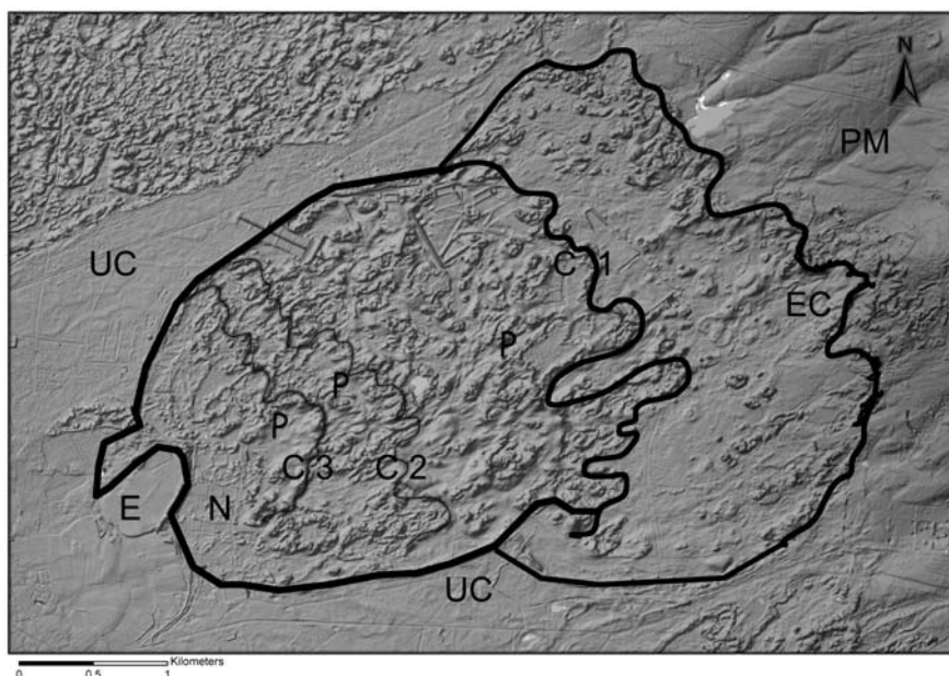
Fig 4. The drift sand cell east of Harskamp , terminating in comb dunes C1 . N indicates the zone of nabkhas; P the deflation planes; C2 and C3 mark the comb dune ridges at various stages of windward expansion. Long before the 19 th century the farmers protected their fields E with a wall, to check SW expansion of the drift sand. UC =unaffected old cover sand separating the Harskampsezand from the other clusters; PM =push moraine ridge; EC =terminating comb dunes of preceding cells. Compiled by M. Riksen, data source: AGI-ITC Rijkswaterstaat, 2004.
