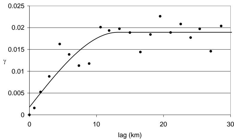
Figure 8. Dots: sample semivariogram of scores observed in ditches, in the sub-catchment Rhine-West, north of the North Sea Canal. Line: the spherical model that has been fitted to the sample semivariogram, with c_0=0.002 , c_1=0.017 , and a=13.216 km.
