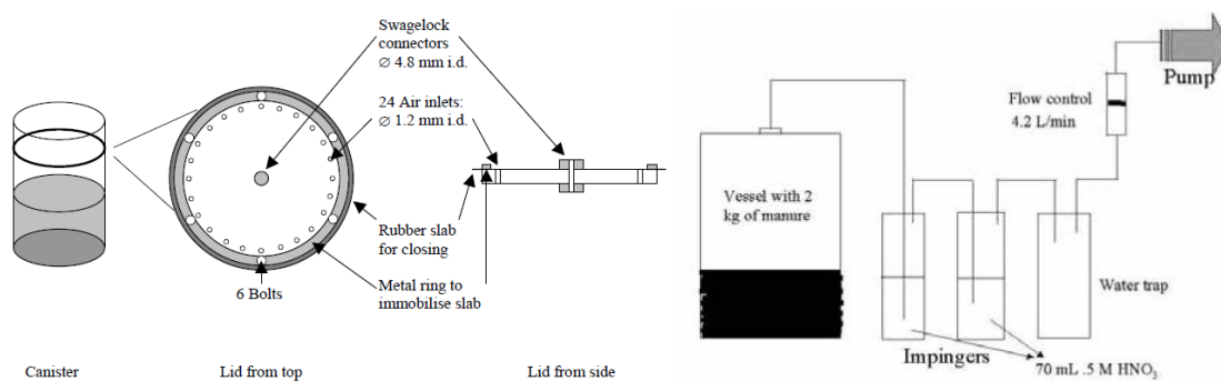
FIGURE 1 Overview (right) of experimental setup for measuring ammonia emissions and detail (left) of the lid of the vessel (=canister).
