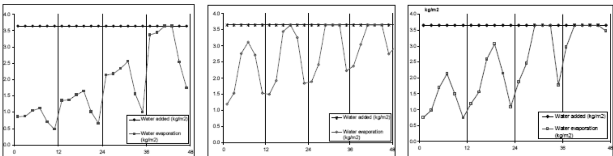
FIGURE 4 Modeled water evaporation ( \text{kg/m}^2 ) without composting in The Netherlands (left), Israel (middle) and Minnesota (right) at airspeeds of 0.08 m/s (0-12 months), 0.32 m/s (12-24 months), 1.28 m/s (34-36 months) and 5.12 m/s (36-48 months).
