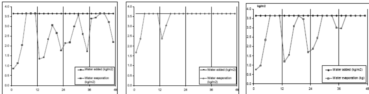
FIGURE 3 Modeled water evaporation ( \text{kg/m}^2 ) with composting for conditions in The Netherlands (left), Israel (middle) and Minnesota (right) at airspeeds of 0.08 m/s (0-12 months), 0.32 m/s (12-24 months), 1.28 m/s (34-36 months) and 5.12 m/s (36-48 months).
