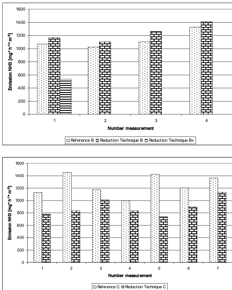
Figure 2. Ammonia emission level of the different reduction systems and paired references per replicated measurement.
