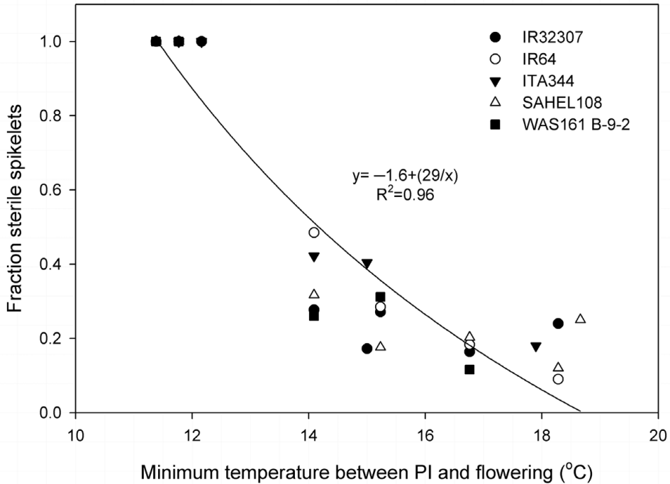
Figure 5. Relation between the minimum temperature between panicle initiation (PI) and flowering stage (°C) and fraction of sterile spikelets for five varieties, grown during months in which no heat stress occurred.
