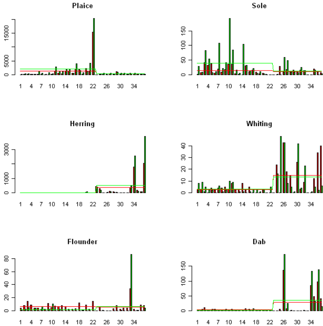
Figure 7. Barplot of the by-catches in the sievenet (green) and letterbox (red) for the successive hauls (x-axes: 1-22: first season; 23-37 second season) of plaice, sole, herring, whiting, flounder and dab in number/hr (y-axes).
