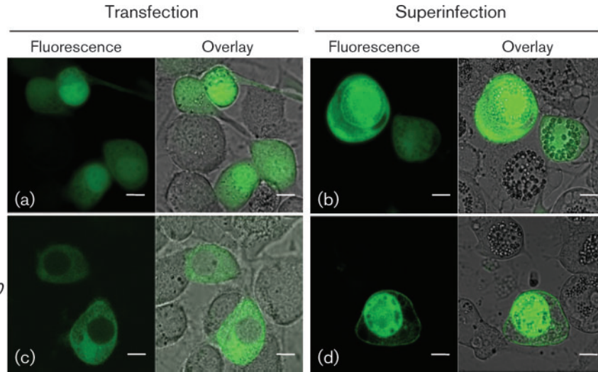
Fig. 2. Subcellular localization of EGFP-fused HA100. Confocal fluorescence analysis was employed to study the localization of the protein in infected cells. HzAM1 cells were transfected with pIZ/V5-egfp (a, b) or pIZ/V5-egfp/ha100 (c, d) followed by superinfection (b, d) with HearNPV. Fluorescent microscopy was performed at 72 h p.i. Left panels are images under fluorescent microscopy and right panels show the overlay results under fluorescent and visible microscopy. Bars, 10 μm.
