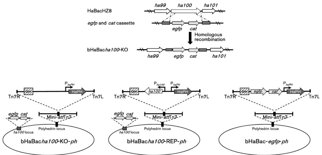
Fig. 3. Construction of recombinant bacmids. The chloramphenicol acetyltransferase ( cat ) and egfp genes flanked by ha100 sequences (57 bp homologous arm) were used for homologous recombination to generate bHaBacha100-KO. The ph gene was reintroduced into bHaBacha100-KO to generate bHaBacha100-KO-ph. The ha100 and ph genes under their native promoters were inserted into the ph locus of HaBachZ8 by Tn7-mediated transposition to generate bHaBacha100-REP-ph. bHaBac-egfp-ph was a control virus containing EGFP as the marker. Gm r , Gentamicin resistance gene.
