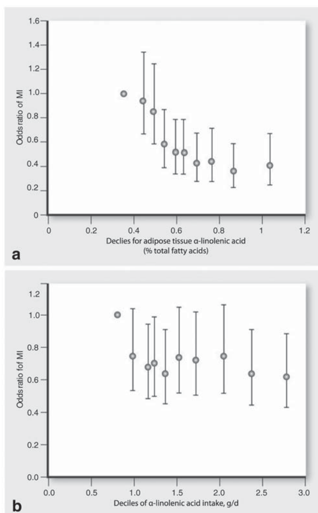
Figure 3.1 Odds ratios and 95% confidence intervals for nonfatal myocardial infarction (MI) by deciles of alpha-linolenic acid in adipose tissue (a) or intake (b) in a case-control study of 3,638 men and women in Costa Rica. Data were adjusted for smoking status, physical activity, household income, history of diabetes mellitus, history of hypertension, waist-to-hip ratio, saturated fat intake, and linoleic and trans -fatty acids in adipose tissue. (From Campos et al., 19 with permission.)
