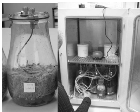
Figure 1: Experimental setup of compost experiments.
