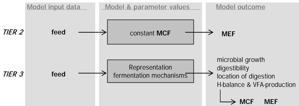
Figure 1. Schematic representation of the difference between the calculation rules (indicated by the grey frames) used in the Tier 2 approach (according to IPCC, 1996) and those used in the Tier 3 approach (according to Mills et al. , 2001, and Bannink et al. , 2008) to determine the MEF (kg CH 4 /cow/year) and MCF (CH 4 as % of the GE intake).
