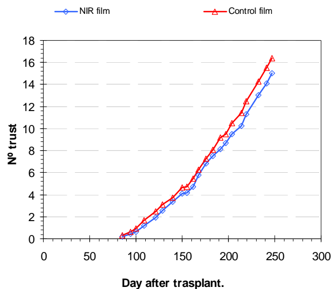
Figure 4.10. Accumulated number of trusses harvested for each treatment along the growing cycle.
