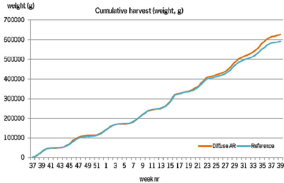
Figure 5.12. Cumulative production in gram harvested product in both compartments.
