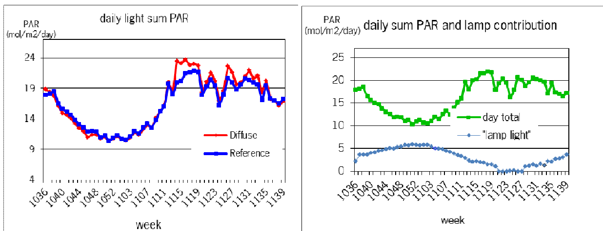
Figure 5.11 (left): Light sum in both greenhouses along the year, and right, contribution of the lamps to the total daylight sum.
