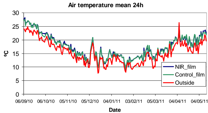
Figure 4.6. Daily mean 24h air temperature (°C) in NIR_film, Control_film and outside.
