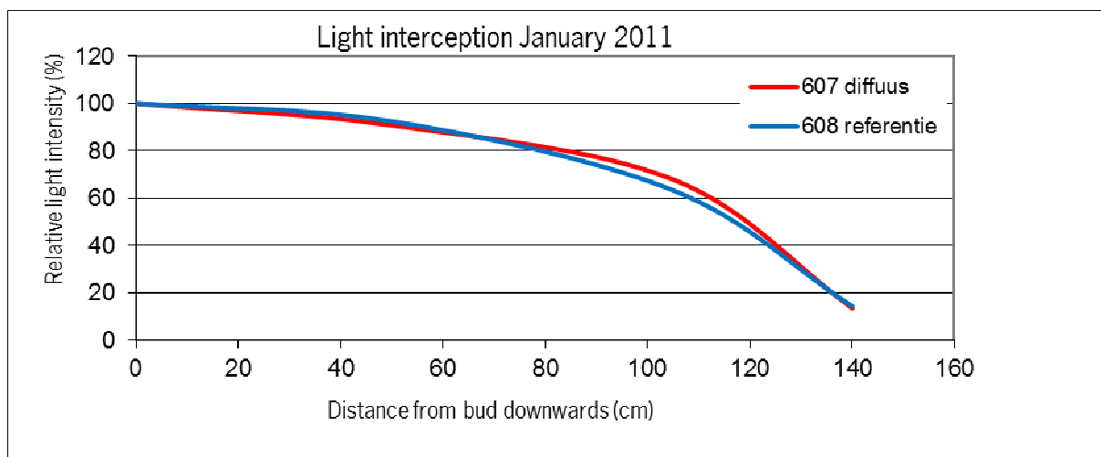
Figure 5.20. Light interception by the crop in January 2011 in both compartments.
