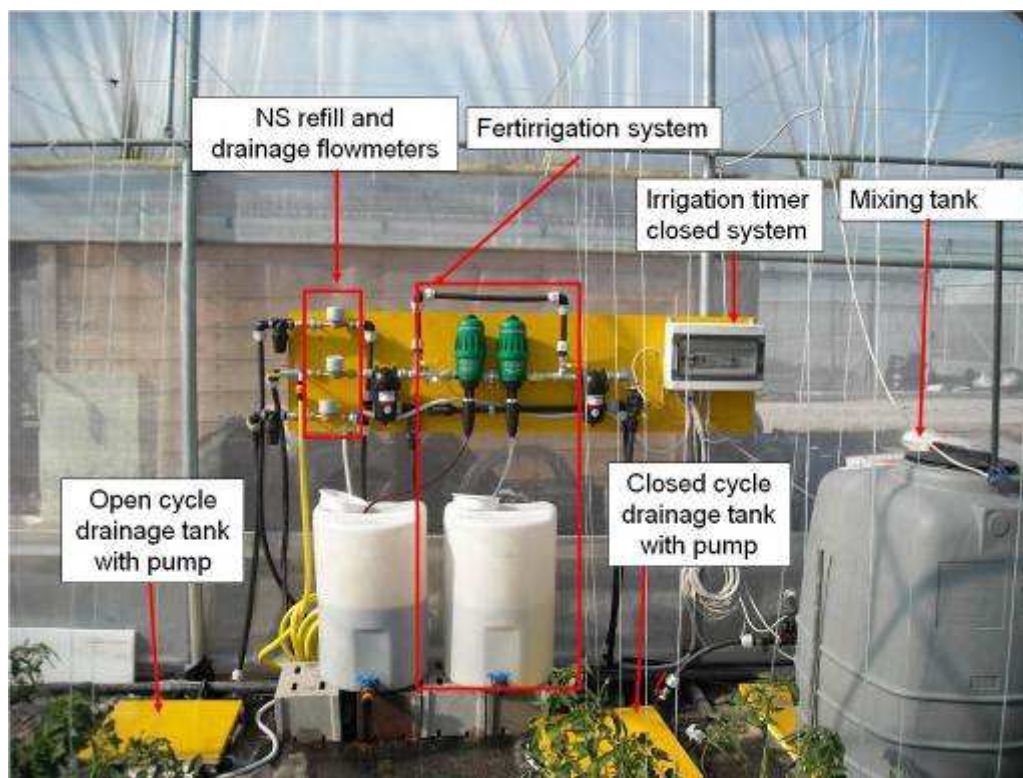
Figure 6.4. The layout of the closed soilless growing system.
