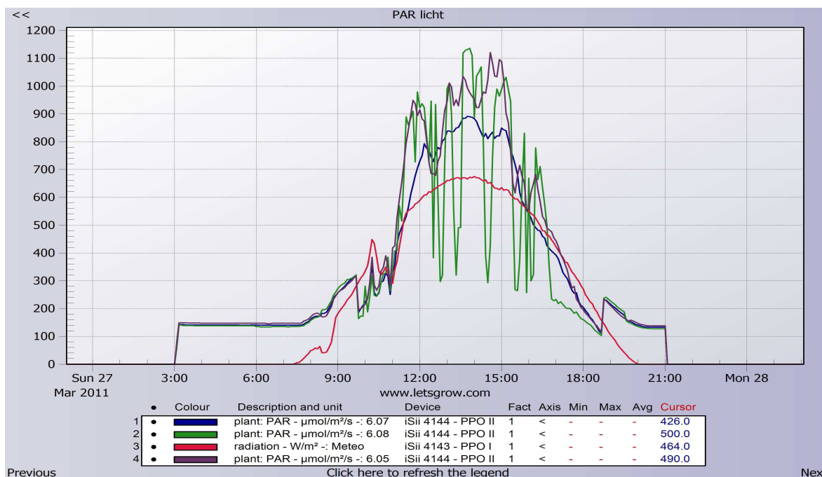
Figure 5.9: Light in three greenhouses with a different glass cover on a sunny day. The red line is the outside radiation, the green line the light in the reference greenhouse. The purple line shows the light in a third greenhouse (diffuse, one side Anti Reflection coating) and the blue line is the greenhouse with diffuse glass with double sided Anti Reflection coating by GroGlass.
