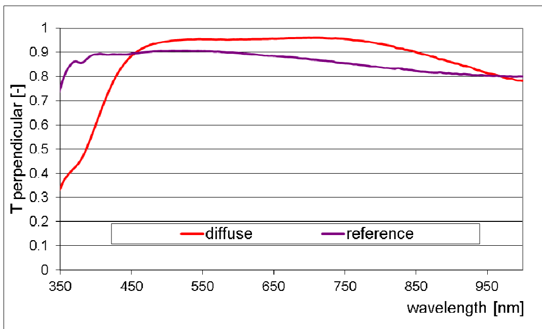
Figure 5.1: Light transmission of the glass (laboratory measurements) as compared to the standard (normal float) glass.
