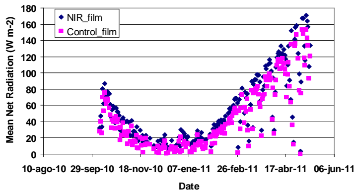
Figure 4.7. Daily mean net radiation (Wm -2 ) over greenhouse for two treatments: NIR and Control.
