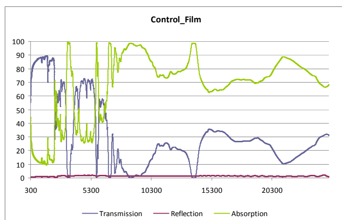
Figure 4.3. Transmission, reflection and absorption spectrum of the two tested materials: NIR_film and Control_film (laboratory data measured and provided by WUR).
