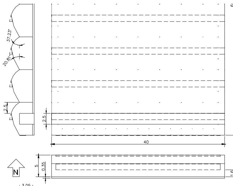
Figure 4.1.- Structure and dimensions of the experimental greenhouse compartments
