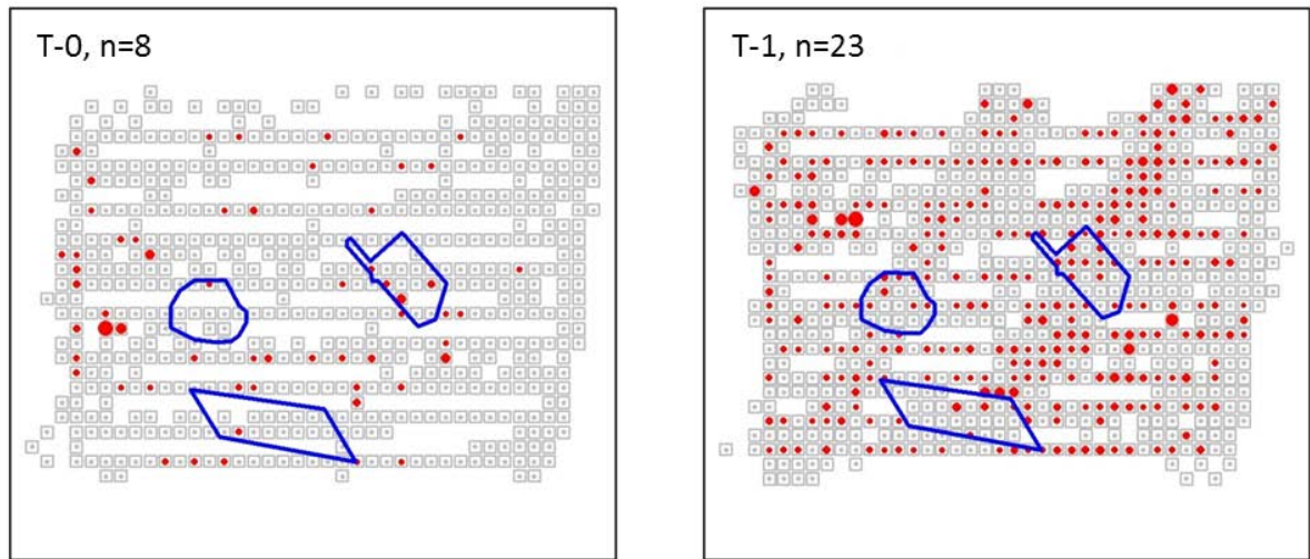
Figure 58. Averaged distribution patterns compared for all T-0 surveys versus all T-1 surveys.
