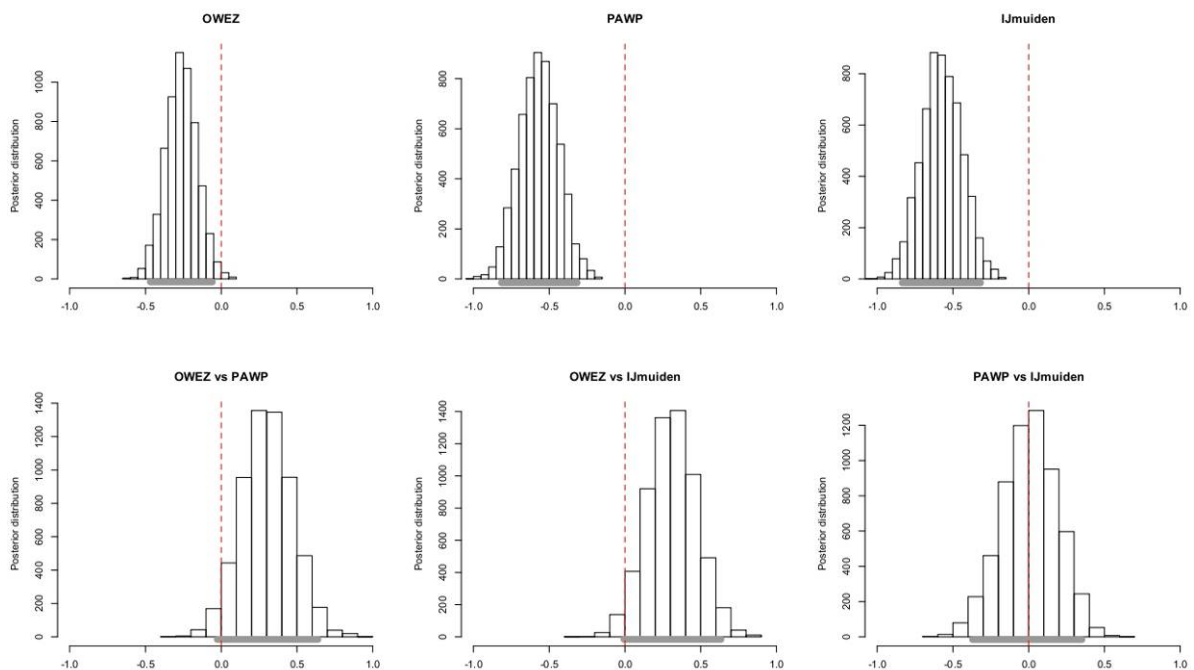
Figure 56. Estimates of parameter coefficients for the three 'disturbance' areas, and the significance of the difference between these areas. If there is no effect of a 'disturbance area', the parameter coefficient would be zero. A significant deviation from zero is reached when zero (the red dotted line) is outside 95% of the parameter coefficient estimates (the grey bars at the bottom of the histograms).
