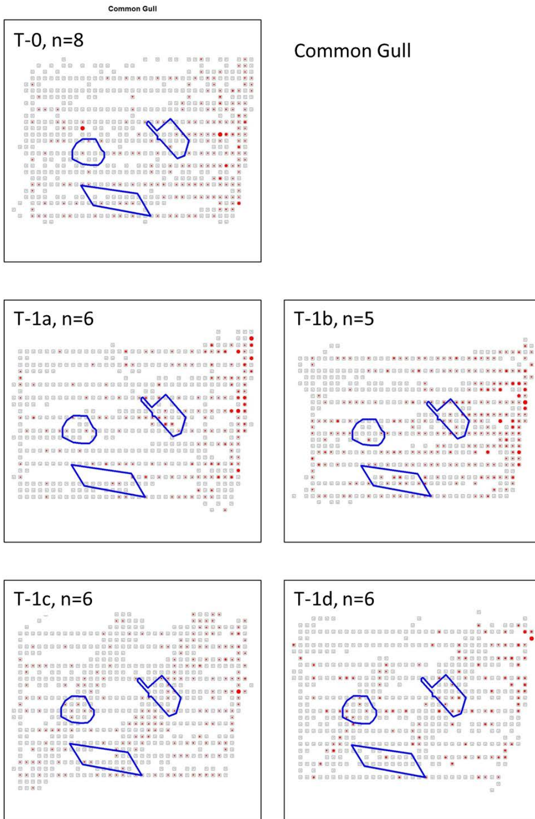
Figure 34. Averaged distribution patterns during the various survey phases.
