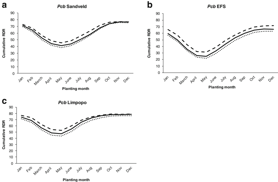
Fig. 4 Cumulative relative development rates (cRDR) of Pectobacterium carotovorum subsp. brasiliensis ( Pcb ) on potatoes for the periods 1961–1970 (dotted line), 2001–2010 (solid line) and 2041–2050 (broken line) in a the Sandveld, b the Eastern Free State (EFS) and c Limpopo growing regions in South Africa
