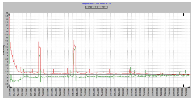
Figure 8, Quest II citrus trial shipment: T_{set} (black), hourly averaged T_{sup} (green) and T_{ret} (red).
