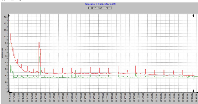
Figure 7, non-Quest citrus trial shipment: T_{set} (black), hourly averaged T_{sup} (green) and T_{ret} (red).
