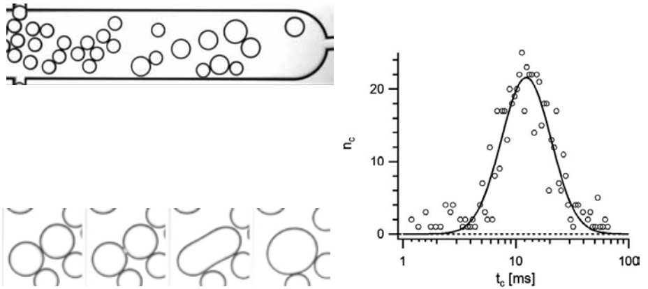
Figure 9. Microfluidic chip with a coalescence chamber for emulsion stability testing (top left image). Bottom left images show four consecutive images showing the coalescence process in detail. Right image, an example of a distribution of coalescence times as measured in the coalescence chamber (Krebs et al, 2012).
