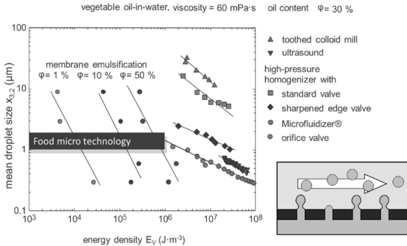
Figure 3. Comparison of various emulsification technologies based on energy density. The graph is adapted from: Schroeder, PhD thesis, TU Karlsruhe. Right bottom insert: principle of cross-flow membrane emulsification; the to-be-dispersed phase is pushed through the membrane and the droplets are sheared off by the cross-flowing continuous phase.
