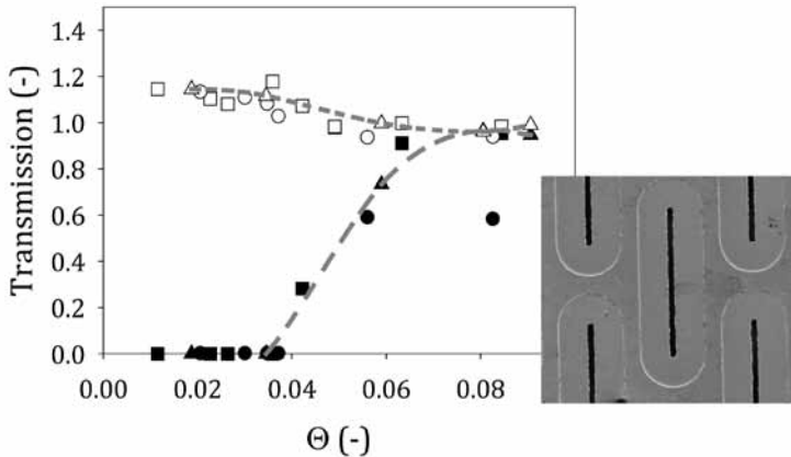
Figure 6. Top. Schematic representation of particle migration in closed channels, with the larger particle moving to the central part and the small ones expelled to the outer regions (Kromkamp et al, 2006). Bottom: Transmission of small (open symbols) and large particles (closed symbols) as function of the dimensionless time ( \Theta ), corresponding to the ratio of transmembrane velocity, and the cross-membrane velocity. The insert shows one of the Stork Veco membranes with uniform pores that were used in the filtrations experiments (van Dinther et al, 2013).
