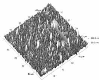
Figure 11. Copper containing microchip for emulsification (left image), and a roughness plot obtained by atomic force microscopy of the same surface (right image) (Maan et al, 2013).
