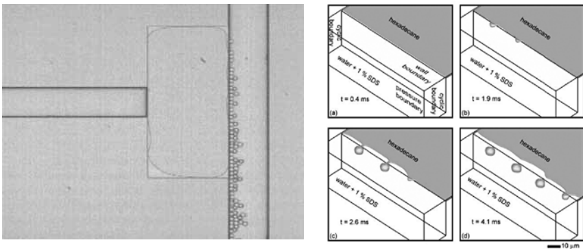
Figure 4. EDGE emulsification as recorded by high speed imaging (left) and by computer simulations (right). The to-be-dispersed phase is pushed onto the shallow wide plateau. Upon reaching the end of the plateau, droplets can expand into a deeper channel where they spontaneously snap off due to (Laplace) pressure differences (van Dijke et al, 2009).
