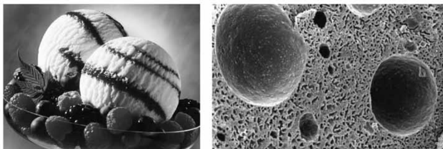
Figure 2. Ice cream, and scanning electron microscopic image of ice cream. The large objects are air bubbles stabilised by small fat crystals, which in turn are surrounded by a protein matrix.
