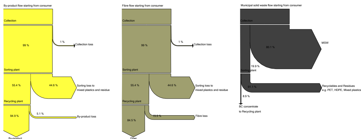
Figure 60 Material flow for the fibre and by-products originating from Schönmackers (left and middle) and for the total MSW originating from Schönmackers (right)
