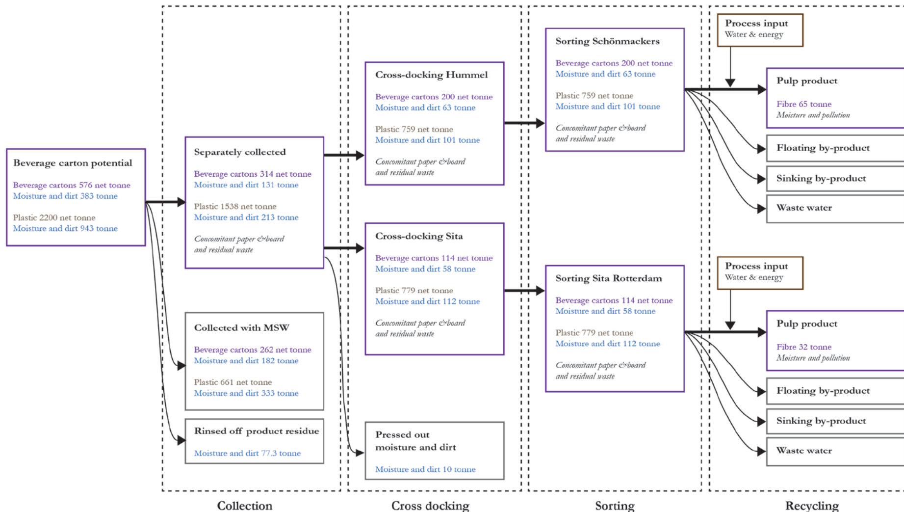
Figure 68: Overview of mass flow diagram for separate collection of beverage cartons
