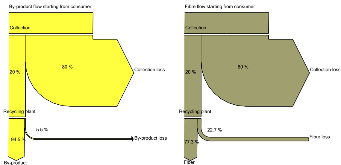
Figure 61 Material flow for the fibre and by-products originating from the separate collection of BC
