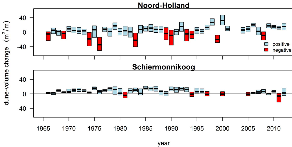
Figure 3. Temporal variability in dune-volume changes. Range of dune-volume changes ( \Delta V ) per year, calculated for Noord-Holland (top) and Schiermonnikoog (bottom). Each boxplot represents the upper and lower quartile and median of dune-volume changes for a single year. Differences among years indicate temporal variability in dune-volume changes. The height of the boxes indicates spatial variability in dune-volume changes. Boxes with a positive median are in blue, boxes with a negative median are in red. doi:10.1371/journal.pone.0091115.g003
