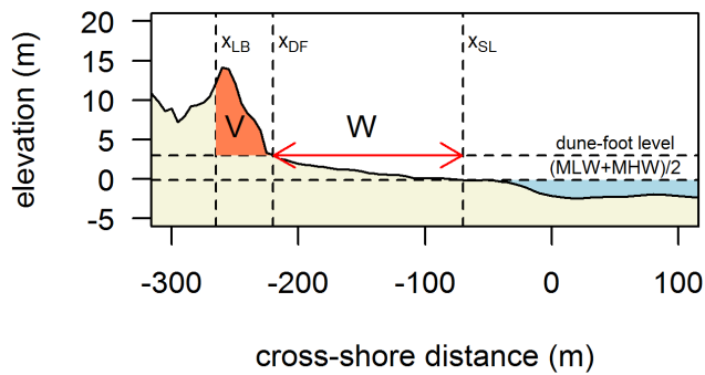
Figure 2. Definition of dune volume and beach width. Position of landward boundary ( X_{LB} ), dune-foot position ( X_{DF} ) and shoreline position ( X_{SL} ) for the black profile. Dune volume ( V ) and beach width ( W ) were calculated on the basis of these positions. doi:10.1371/journal.pone.0091115.g002
