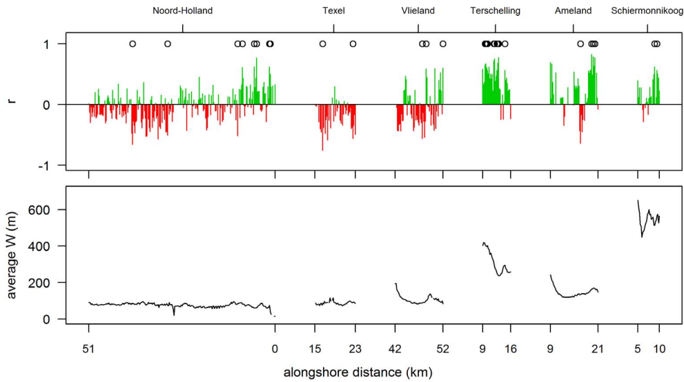
Figure 9. Correlation between time-series of dune-volume changes ( \Delta V ) and transport potential ( Q ). Upper panel: correlation between \Delta V and Q , after discarding years with S > 2.5 m. Correlation was calculated as the Pearson product-moment coefficient r . Correlations significant at p < 0.05 level are indicated with 'o'. Lower panel: time-averaged beach width ( W ) for each profile. The numbers on the x-axis refer to the boundaries of each location. doi:10.1371/journal.pone.0091115.g009
