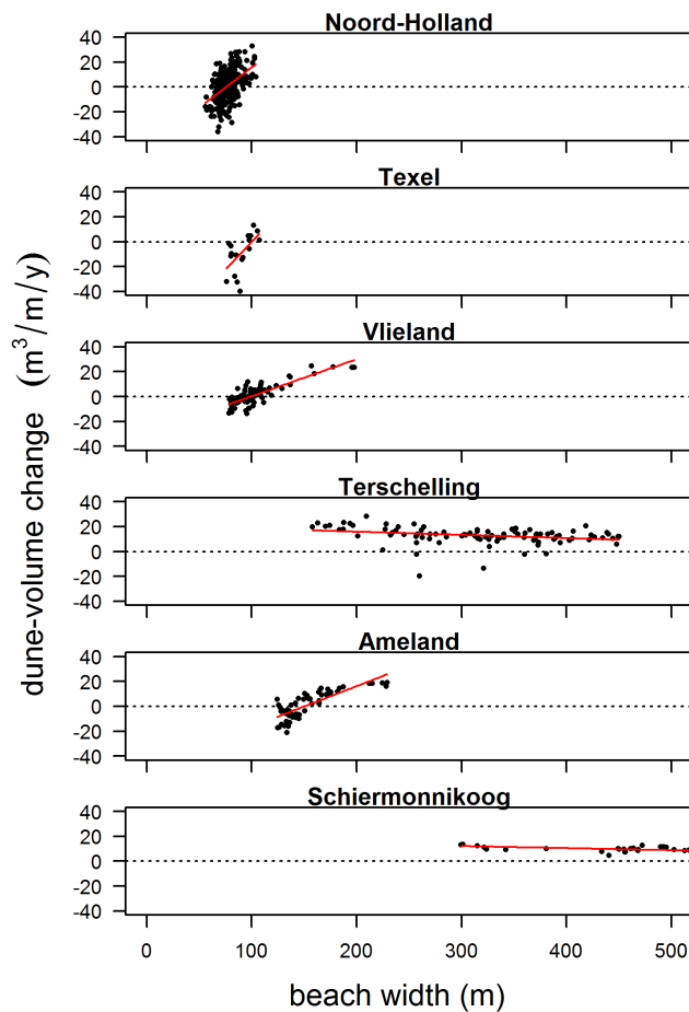
Figure 11. Decadal dune-volume changes ( \Delta V ) as a function of 10-y-averaged beach width ( W ). Red line indicates least-squares linear fit. All correlations are significant at the p < 0.05 level. Values representing a profile with nourishment activity within the specific decade were discarded. doi:10.1371/journal.pone.0091115.g011
