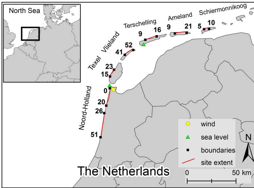
Figure 1. Study areas. Map shows the location of the six coastal sections used in this study within the Netherlands and identifies the location of the wind gauge (KNMI station De Kooy) and two sea-level gauges (Den Helder and West Terschelling). Positions and numbers of beach poles on the section boundaries are indicated. Inset shows the location of the study area within Northwestern Europe. doi:10.1371/journal.pone.0091115.g001
