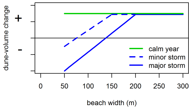
Figure 12. Schematic illustration of the influence of storminess and beach width on foredune volume. When beach widths are less than 200 m, \Delta V depends on storminess. When beach width is over 200 m, as occurs e.g. on Terschelling and Schiermonnikoog, \Delta V is no longer dependent on storminess or beach width. doi:10.1371/journal.pone.0091115.g012
