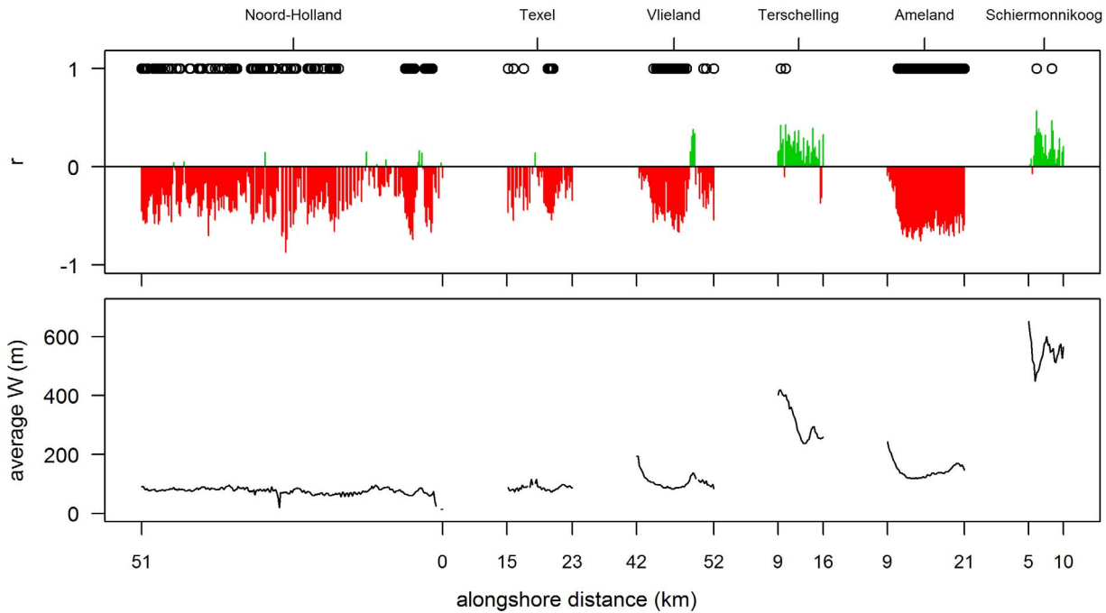
Figure 7. Temporal correlation of dune-volume changes ( \Delta V ) and storminess ( S ). Upper panel: correlation between dune-volume changes ( \Delta V ) and storminess ( S ). Correlation was calculated as the Pearson product-moment coefficient r . Correlations significant at p < 0.05 level are indicated with 'o'. Lower panel: time-averaged beach width ( W ) for each profile. The numbers on the x-axis refer to the boundaries of each location. doi:10.1371/journal.pone.0091115.g007
