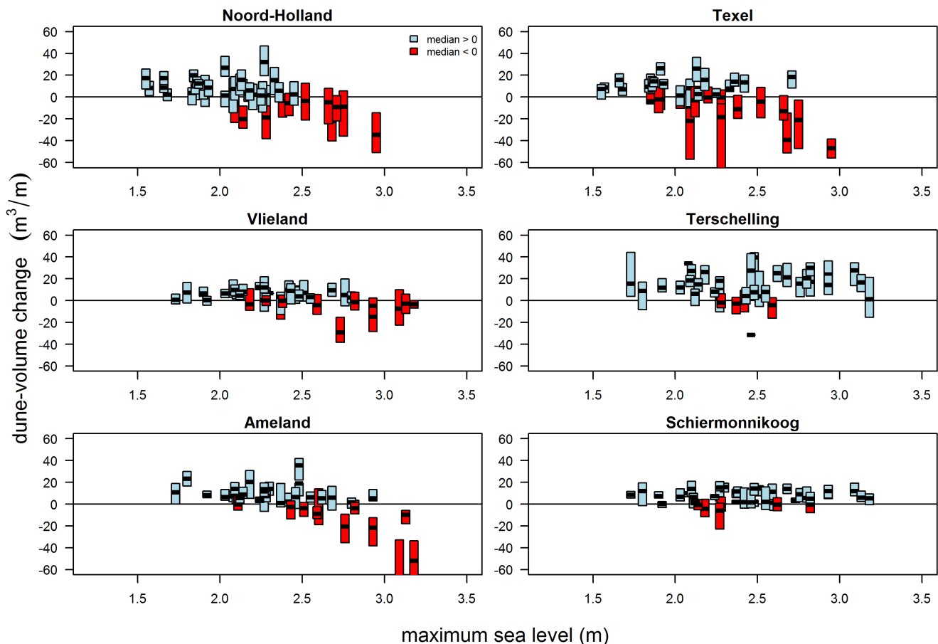
Figure 6. Dune-volume changes ( \Delta V ) as a function of maximum sea level ( S ) for all sites. Each boxplot represents the longshore variation for a single year. Boxplots with a positive median in blue, with a negative median in red. doi:10.1371/journal.pone.0091115.g006
