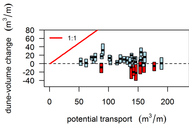
Figure 8. Dune-volume changes ( \Delta V ) as function of transport potential for Noord-Holland. Each boxplot represents the alongshore variation of a single year. Boxplots with a positive median in blue, boxplots with a negative median in red. The red line indicates the 1:1 line, where potential transport equals \Delta V . doi:10.1371/journal.pone.0091115.g008
