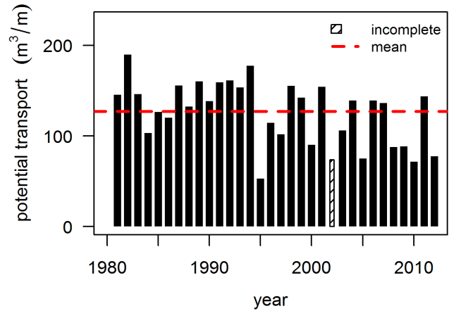
Figure 5. Yearly transport potential. Yearly transport potential for location Noord-Holland. The measurements of 2002 are incomplete, with 22 hours of missing data. This hiatus seems unrelated to storm conditions. The mean transport potential is 125 \text{ m}^3/\text{m} . doi:10.1371/journal.pone.0091115.g005
