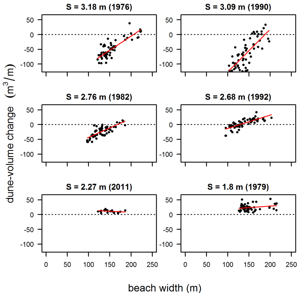
Figure 10. Correlation between dune-volume change ( \Delta V ) and beach width ( W ) for different values of storminess ( S ). Data from section Ameland. The red line represents the least squares linear regression. doi:10.1371/journal.pone.0091115.g010
