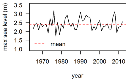
Figure 4. Yearly maximum sea level. Yearly maximum sea level as measured at the tide station of West-Terschelling (1965–2012). doi:10.1371/journal.pone.0091115.g004
