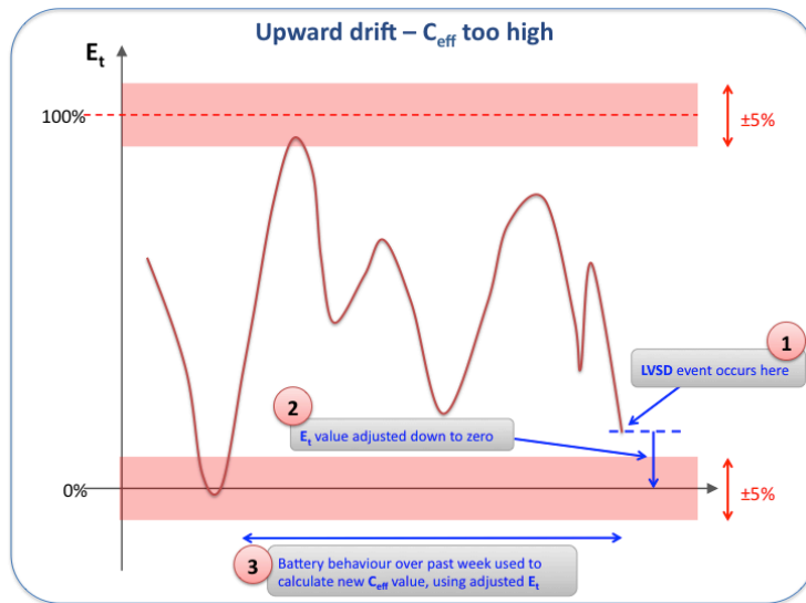
Figure 8: Upward drift of calculated charge level caused by the charge efficiency value, C_{eff} , being too high, and the correction of this drift.
