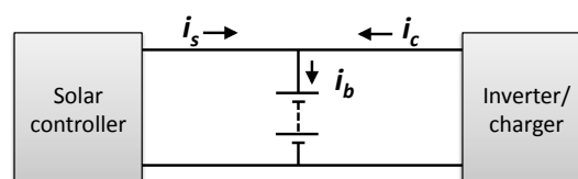
Figure 3: Neither the inverter/charger nor the solar controller can independently determine the actual battery current, i_b .
