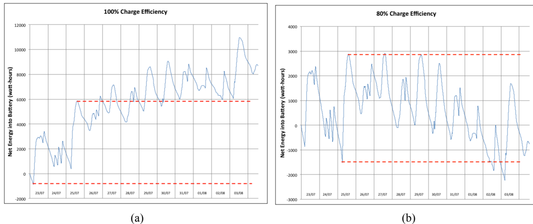
Figure 7: Net energy into the batteries (effectively energy stored) from the data of Figure 6, assuming (a) an overall charge/discharge efficiency ( C_{\text{eff}} ) of 100%, and (b) an efficiency of 80%.
