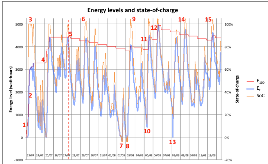
Figure 12: Algorithm and parameter development based on the 3 week sample data, showing battery stored energy E_t , battery maximum capacity E_{100} , and state-of-charge SoC . The overlaid numbers indicate notable points which are described in the text.
