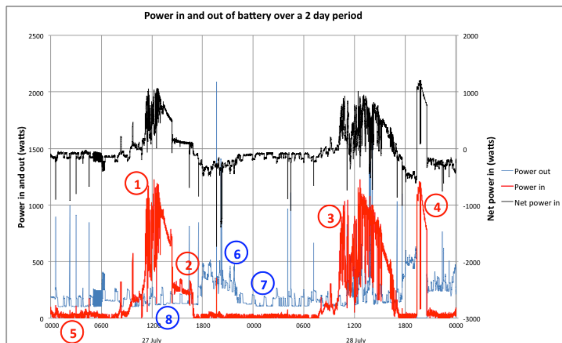
Figure 5: Detail of power in and out of the Pauaekē batteries over two days, showing the cyclic nature of both consumption and generation.
