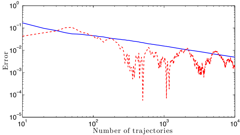
FIG. 4: Statistical errors in the quantum trajectories computation for a two-level system. Here we compare the statistical error estimate (blue solid line) to the absolute error in the averaged value of P_e when compared with the exactly computed value (red dashed line) at a time t\Omega = 40 . We show these values as a function of the number of trajectories over which we average, with all quantities plotted on a logarithmic scale. As expected, the behaviour of both the statistical error and the discrepancy is somewhat erratic for small numbers of trajectories, but decrease steadily \propto 1/\sqrt{N} for larger numbers. The absolute error is mostly below the statistical error estimate, consistent with a gaussian distribution of possible errors with a standard deviation equal to our statistical error estimate. Note that these values depend on the particular random sample of trajectories obtained in the calculation. From the central limit theorem and the properties of Gaussian distributions that for any given computed values, we expect the absolute error to be smaller than the statistical error as it is quoted here for 68.2% of all possible samples.
