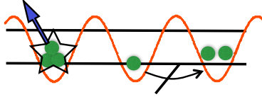
FIG. 23: Schematic showing the continuous quantum Zeno effect in the case of three-body loss in an optical lattice. If we have a large on-site rate of loss \gamma_3 , such that the tunnelling in the lowest Bloch band J \ll \gamma_3 , then tunnelling processes that populate a single site with three particles (i.e., where a particle on one site tunnels onto an already doubly-occupied site) will be suppressed. In this form, large on-site loss rates can counterintuitively lead to a reduction in the overall rate of loss, and can act as an effective dynamical interaction, which suppresses triple occupation.
