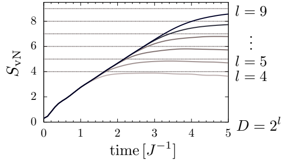
FIG. 10: Increase in entanglement as a function of time after a quantum quench in the Bose-Hubbard model. Here we consider a quench in the Bose-Hubbard model eq. (48) from U = 10J to U = J in a system with 30 particles on 30 lattice sites, initially in the ground state with U = 10J . Making a bipartite splitting in the centre of the system (with 15 sites on each side), we compute the von Neumann entropy increase as a function of time using t-DMRG methods with varying values of D . We see clearly the bounds in S_{\text{vN}} imposed by different values of D , which are indicated with dotted horizontal lines, as well as clear convergence of the results at short times to the exact value as we increase D . Adapted from A. J. Daley, H. Pichler, J. Schachenmayer, and P. Zoller, Phys. Rev. Lett. 109 , 020505 (2012).
