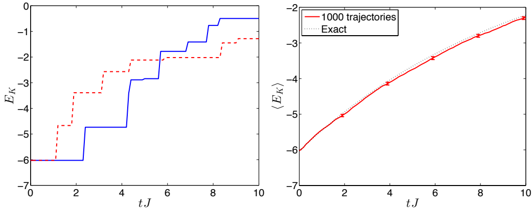
FIG. 5: Illustrative example of quantum trajectories averaging for a gas of hard-core bosons on a lattice, analogous to the example for a two-level system in Fig. 3. Here we show results from exact diagonalisation calculations with 5 particles on 10 lattice sites. (left) Kinetic energy of the system of hard-core bosons as a function of time tJ for two example trajectories (with blue solid and red dashed lines showing different random samples). We see the effect of quantum jumps, where the kinetic energy increases as individual atoms are localised in space, and hence spread over the Brillouin zone in quasi-momentum. Here the scattering rate \Gamma = 0.1J . (right) Values for the kinetic energy averaged over 1000 sample trajectories, compared with the exact result from eq. (51). As in the case of the two-level system, the quantum trajectories results agree with the exact results within the statistical errors, which are shown here as error bars calculated as described in section III C.
