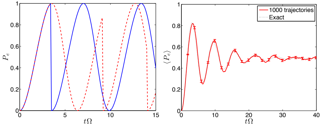
FIG. 3: Illustrative example of quantum trajectories averaging for a two-level system. (left) Probability of finding the atom in the excited state P_e as a function of time t\Omega for two example trajectories (with blue solid and red dashed lines showing different random samples). We see the effect of quantum jumps, where the atom is projected on the ground state. Here the detuning \Delta = 0 , and \Gamma = \Omega/6 . (right) Values for P_e averaged over 1000 sample trajectories (Solid line), compared with the exact result from direct integration of the master equation (dotted line). The quantum trajectories results agree with the exact results within the statistical errors, which are shown here as error bars calculated as described in section III C.
