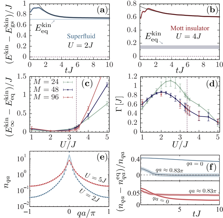
FIG. 20: Time evolution after a single spontaneous emission (averaged over jumps on all possible sites). (a - b) For a superfluid initial state ( U = 2J ), the kinetic energy relaxes to the equilibrium value obtained from a Quantum Monte Carlo (QMC) calculation E_{\text{eq}}^{\text{kin}} . For MI states ( U = 4J ), the energy relaxes, but not to E_{\text{eq}}^{\text{kin}} . The zero value of kinetic energy for this plot is the ground state kinetic energy E_{\text{gs}}^{\text{kin}} . (c) The difference of the infinite time value of the kinetic energy (obtained from an extrapolation of an exponential fit) to the Monte Carlo equilibrium energy. For MI states with U/J \gtrsim 3.37 , the difference increases rapidly for system sizes M = 24, 48, 96 sites (d) The decay rate extracted from the exponential fit as a function of U . (e) Comparison of the time-evolved quasi-momentum distribution at t = 10/J (dots) to the equilibrium distribution from a QMC calculation. (f) Differences between the two distributions as a function of time for the qa = 0 peak and for a large quasi-momentum of qa = (40/48)\pi . In the superfluid ( U = 2J ), the components for large momenta relax rapidly to thermal values, for qa \sim 0 , the relaxation timescale is much longer. In the MI with U = 5J , the same is true, but for large momenta there is a discrepancy to the thermal value. (t-DMRG results, d_i = 6 , D = 256, 512 ; error bars represent fitting errors and statistical errors from QMC. Reprinted figure from J. Schachenmayer, L. Pollet, M. Troyer, and A. J. Daley, Phys. Rev. A 89 , 011601(R) (2014) [86]. Copyright 2014 by the American Physical Society.
