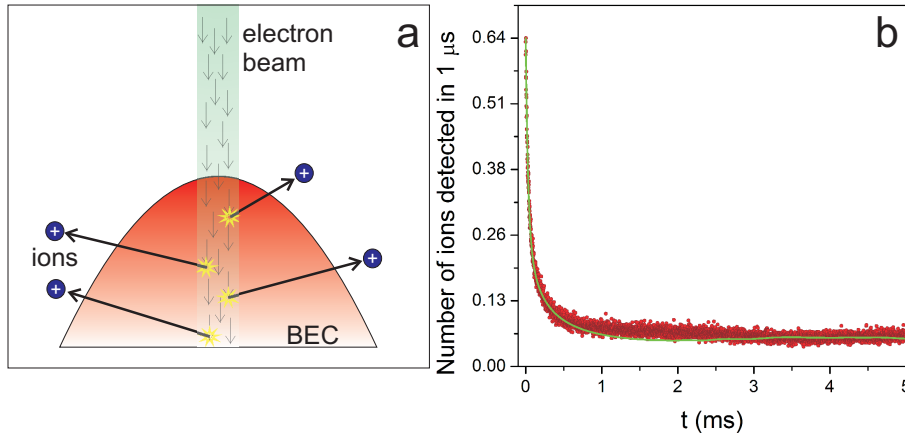
FIG. 26: a) The electrons locally collide with the atoms constantly dissipating the BEC. b) Temporal resolved signal from the ion detector. The bin size is 1 \mu\text{s} . Points are experimental data averaged over 1800 experimental repetitions, while the solid curve is the numerical simulation (see text). After 5 ms we typically collect \simeq 450 ions. Reprinted figure with permission from G. Barontini, R. Labouvie, F. Stubenrauch, A. Vogler, V. Guarrera, and H. Ott, Phys. Rev. Lett. 110 , 035302 (2013). Copyright 2013 by the American Physical Society.
