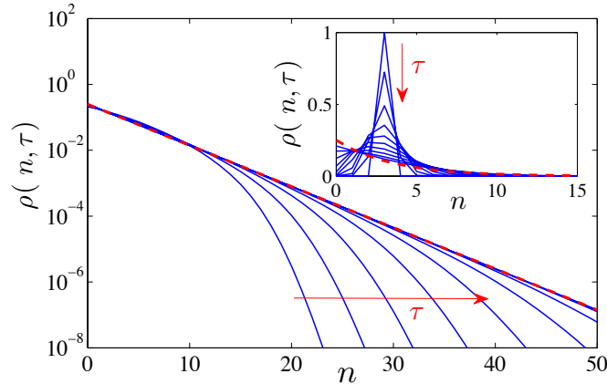
FIG. 18: Numerical evolution of the density matrix elements \rho(n, \tau) (solid lines), where the density operator is given by the ansatz \bigotimes_j [\sum_n \rho(n, t)|n\rangle\langle n|] , in a semi-logarithmic plot, versus n for large rescaled times \tau between 0.1 and 50 (not equidistant) in the direction of the (red) arrow. The inset shows the same evolution at shorter times \tau between 0.0002 and 0.1 (not equidistant) in the direction of the (red) arrow in a linear plot. Parameters: N/L = 3 , U/\hbar\gamma = 10 . The (red) dashed lines show the (analytical) asymptotic limit. Reprinted figure with permission from D. Poletti, P. Barmettler, A. Georges, and C. Kollath, Phys. Rev. Lett 111 , 195301 (2013) [83]. Copyright 2013 by the American Physical Society.
