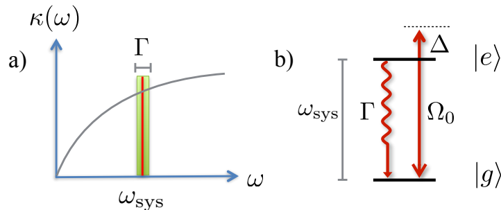
FIG. 2: (a) Coupling constant as a function of frequency, \kappa(\omega) , illustrating a slowly varying coupling strength around the central system frequency \omega_{\text{sys}} . This is a key to several of the approximations made for open quantum systems in quantum optics. (b) Comparison of the scales for a two-level system. The system frequency is the optical frequency, \omega_{\text{sys}} , associated with the energy difference between the ground and excited levels. In order to make the standard approximations, we require the timescale for the decay of the excited state, \Gamma^{-1} , i.e., the timescale for the dynamics induced by coupling to the environment, to be much longer than the optical timescale associated with the transition, or in frequency units, \Gamma^{-1} \gg \omega_{\text{sys}}^{-1} . We also work in a limit where any remaining system dynamics are associated with much smaller frequency scales. In this case, the coupling strength \Omega_0 , associated with the frequency of Rabi oscillations between the states when they are coupled strongly on resonance, as well as the frequency of detuning from resonance \Delta , satisfy \Omega_0, \Delta \ll \omega_{\text{sys}} .
