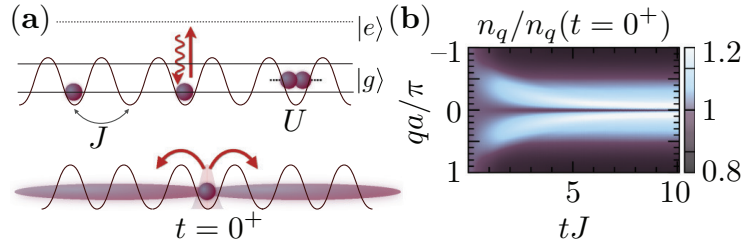
FIG. 19: (a) Absorption and spontaneous emission of a lattice photon leads effectively to localization of single atoms. Tunnelling and interactions between atoms then redistribute the energy added to the system. (b) Localization of an atom in space corresponds initially to a distribution of the atom over the whole Brillouin zone (the tails of the quasi-momentum distribution are lifted). Subsequent unitary evolution leads to a broadened quasi-momentum distribution, i.e. , the n_{q=0} peak and the tails decrease, while the small quasi-momentum components increase (t-DMRG results, U = 2J , N = 48 particles on L = 48 sites, d_l = 6 , D = 512 ). Reprinted figure from J. Schachenmayer, L. Pollet, M. Troyer, and A. J. Daley, Phys. Rev. A 89 , 011601(R) (2014) [86]. Copyright 2014 by the American Physical Society.
