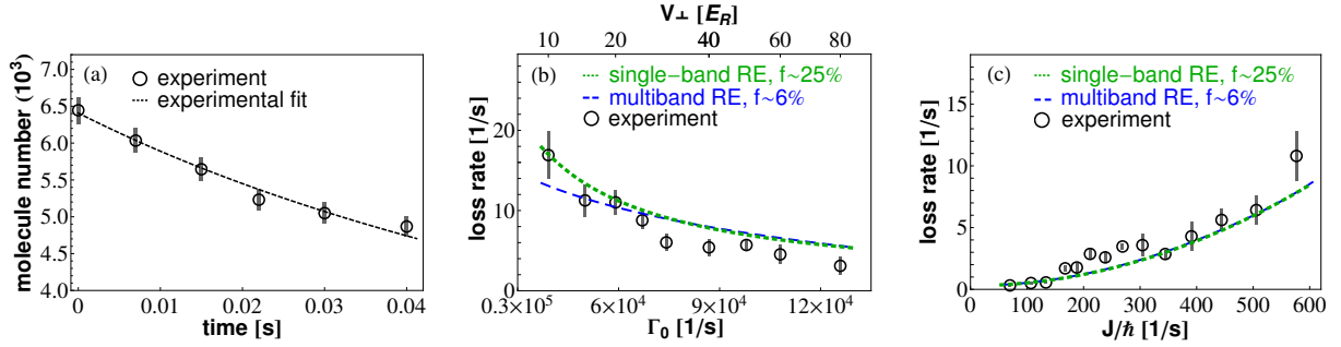
FIG. 22: (a) Measured number loss of |\downarrow\rangle molecules for an axial (transverse) lattice depth of V_y = 5 E_R ( V_\perp = 25 E_R ) (circles) and best fit using a rate equation, dN_\downarrow/dt = -\kappa N_\downarrow(0)/[N_\downarrow(t)]^2 (black dashed line). (b) Number loss rate, \kappa , as a function of \Gamma_0 (fixing J \approx 570 Hz and varying the bare on-site rate via V_\perp ). (c) Number loss rate, \kappa , versus J for fixed \Gamma_0 \approx 87 kHz (varying V_y and adjusting V_\perp accordingly). V_y ( V_\perp ) was varied from 5 to 16 E_R (20 to 40 E_R ). Black circles are experimental measurements (error bars represent one standard error). Green short-dashed lines show solutions of the rate equation using an effective loss rate \Gamma_{\text{eff}} \propto J^2/\Gamma_0 (single-band approximation). The blue long-dashed line shows the multiband rate equation using \tilde{\Gamma}_{\text{eff}} \propto \tilde{J}^2/\tilde{\Gamma}_0 , in which \tilde{J} and \tilde{\Gamma}_0 are renormalized coefficients based on the effective multi-band theory. The multiband and single-band rate equation results were obtained by fixing the filling fraction to be 6%, and 25% respectively. Panels (b) and (c) directly manifest the continuous quantum Zeno effect: in (b) the measured loss rate \kappa decreases with increasing on-site \Gamma_0 ; in (c) a fit to the experimental data supports \kappa \propto J^2 , with a \chi^2 (sum of the squared fitting errors) several times smaller than for a linear fit. Reprinted figure with permission from B. Zhu et al., Phys. Rev. Lett. 112 , 070404 (2014). Copyright 2014 by the American Physical Society.
