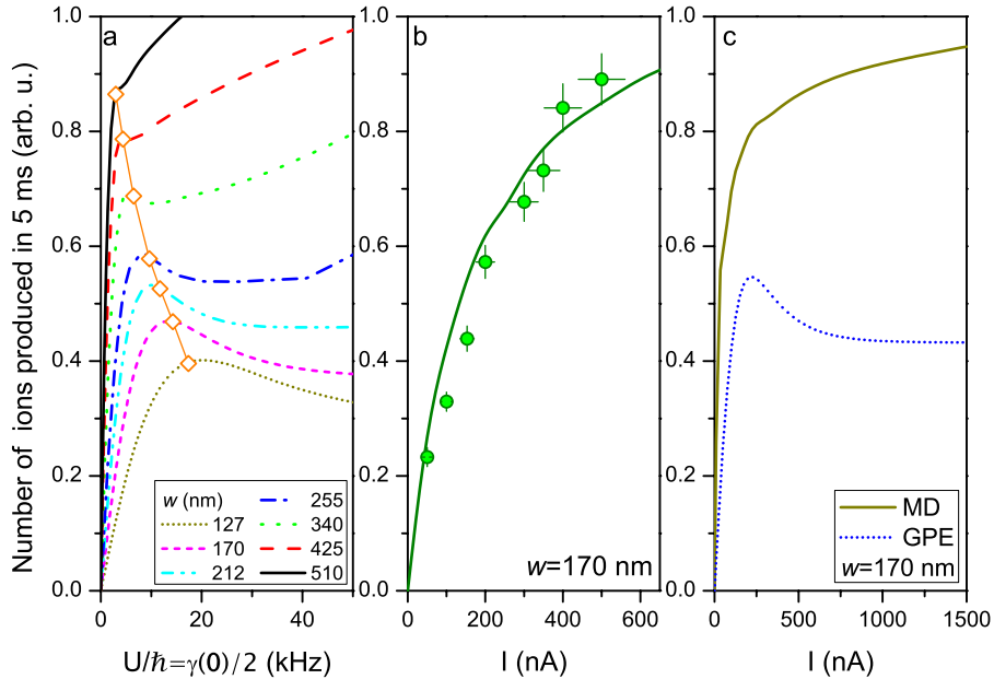
FIG. 27: a) Theoretical curves of the number of ions produced in 5 ms as a function of U/\hbar = \gamma_1(\mathbf{0}) solving equation (84) for different values of the beam width w [122]. The values of U_M obtained using the approximate expression given in the text are shown as open diamonds over the corresponding curves. b) Number of ions measured after 5 ms of dissipation for a thermal cloud as a function of the EB current, with beam width w = 170(7) nm. The solid line is the result of the corresponding numerical simulation using the molecular dynamics method. c) Comparison between the theoretical curves of the number of produced ions as a function of I for the BEC and the corresponding classical analogue (beam width w = 170(7) nm) [122]. Reprinted figure with permission from G. Barontini, R. Labouvie, F. Stubenrauch, A. Vogler, V. Guarrera, and H. Ott, Phys. Rev. Lett. 110 , 035302 (2013). Copyright 2013 by the American Physical Society.
