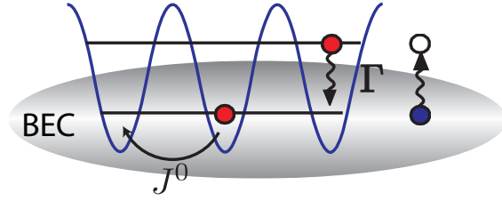
FIG. 28: Schematic picture of atoms in an optical lattice immersed in a Bose-Einstein condensate of another species that is not trapped by the lattice. Processes in which an atom in an excited band of the lattice decays to the lowest band are generated by spontaneous emission of Bogoliubov excitations in the condensate. This process is analogous to spontaneous emissions of photons, but takes place on much smaller energy and momentum scales, allowing for tools such as laser cooling and optical pumping to be reworked in a new context. Figure adapted from A. Griessner, A. J. Daley, S. R. Clark, D. Jaksch, and P. Zoller, New J. Phys 9 , 44 (2007).
