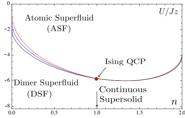
FIG. 24: Phase diagram for the Bose-Hubbard model with a three-body hard-core constraint, and U < 0 . The black curve represents the mean-field phase border, while red (light gray) and blue (dark gray) curves include shifts due to quantum fluctuations in d = 2, 3 . An Ising quantum critical point is predicted in the vicinity of unit filling. The continuous supersolid is reached asymptotically at unit filling. Reprinted figure from S. Diehl, M. Baranov, A. J. Daley, and P. Zoller, Phys. Rev. Lett 104 , 165301 (2010). Copyright 2010 by the American Physical Society.
