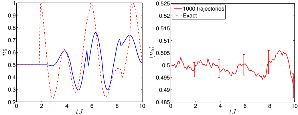
FIG. 7: Illustrative example of quantum trajectories averaging for a gas of hard-core bosons on a lattice, showing results from exact diagonalisation calculations with 5 particles on 10 lattice sites, as in Fig. 5. (left) Density on site 5 of the lattice as a function of time tJ for two example trajectories (with blue solid and red dashed lines showing different random samples). We see the effect of quantum jumps, where nearby jumps give rise to fluctuations either up or down of the local mean density. (right) Values for \langle n_5 \rangle averaged over 1000 sample trajectories, and compared with the exact result, which is \langle n_5 \rangle \equiv \langle a_5^\dagger a_5 \rangle = 0.5 , because the equations of motion are homogeneous. We see that the deviation from this value is well approximated by the statistical errors, shown here as error bars calculated as described in section III C.
