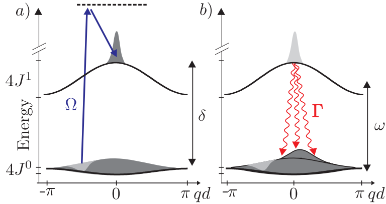
FIG. 29: Schematic picture of one excitation and decay step in Raman cooling in an optical lattice. (a) Atoms are transferred from a region with high quasi-momentum |q| > 0 in the lowest Bloch band to the first excited band. (b) The collisional interaction with the Bose-Einstein condensate atoms is switched on, the resulting decay of the excited lattice atoms leads to a randomization of the quasi-momentum. Sequences of pulses, each one followed by a decay time \tau_c , efficiently excite all atoms outside a narrow region around q = 0 . Repeating the sequence leads to accumulation of atoms in the dark state region around q = 0 , i.e., to cooling. Reprinted figure from A. Griessner, A. J. Daley, S. R. Clark, D. Jaksch, and P. Zoller, New J. Phys 9 , 44 (2007). Copyright 2007 by IOP Publishing Ltd and Deutsche Physikalische Gesellschaft.
