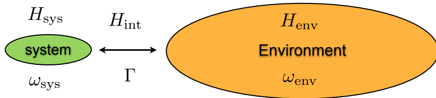
FIG. 1: General framework for an open quantum system: A small quantum system interacts with its environment, leading to a combination of coherent and dissipative dynamics for the small system. In quantum optics, and atomic, molecular, and optical (AMO) systems more generally, the resulting dynamics can both be microscopically well understood, as well as controlled to engineer dynamics or specific quantum states. This involves a separation of energy and frequency scales, where the energy and frequency scales of the small system that are directly coupled to the environment ( \omega_{\text{sys}} ) and the relaxation rates for relevant correlation functions in the environment ( \omega_{\text{env}} ) are much larger than the frequency scales of dynamics induced by the coupling ( \Gamma ).
