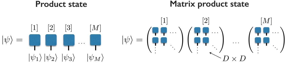
FIG. 8: Diagram comparing a product state and a matrix product state. Each square represents a state |\psi_l\rangle_{[l]} in a local Hilbert space \mathcal{H}_l , e.g., a single spin or lattice site, and the vertical leg on each square box indicates an index for the states of the local Hilbert space. The Hilbert space representing the whole system is the tensor product \mathcal{H} = \mathcal{H}_1 \otimes \mathcal{H}_2 \otimes \dots \otimes \mathcal{H}_L . A product state can be written as |\psi_1\rangle_{[1]} \otimes |\psi_2\rangle_{[2]} \otimes \dots \otimes |\psi_L\rangle_{[L]} , and represents a quantum state with no entanglement between any two local Hilbert spaces. By multiplying out D \times D matrices, a matrix product state makes it possible to represent superpositions of product states, and this superposition contains entanglement between the local Hilbert spaces. For sufficiently large D , any state can be represented in this way, and the ground states of large classes of local 1D many-body Hamiltonians can be represented faithfully for small D in this fashion. This is the basis of the time-dependent density matrix renormalization group method, as discussed in the main text. The maximum amount of entanglement we can represent across any bipartite splitting in the system is bounded in terms of the von Neumann entropy by S_{vN} \leq \log_2 D . Note that while each square box here is a similar notation to that used in Ref. [225] and similar references, in the notation of those references, contractions between matrices are represented by connecting boxes with horizontal lines.
