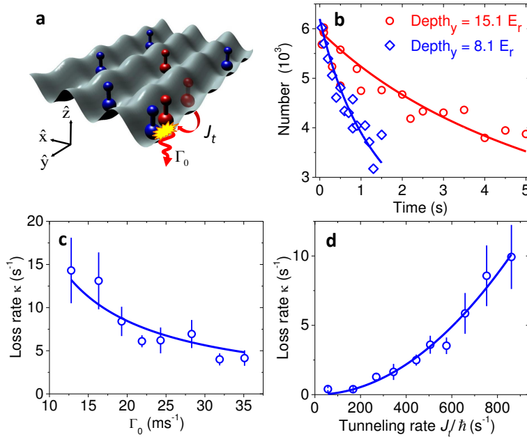
FIG. 21: Quantum Zeno effect for polar molecules in a 3D lattice. a , The lattice depths along x and z are kept at 40 E_R , while the lattice depth along y is reduced to allow tunneling along the y direction at a rate J_t/\hbar . Once two molecules in different spin states tunnel to the same site, they are lost due to chemical reactions at a rate \Gamma_0 . b , Number loss of |\downarrow\rangle state molecules versus time is shown for lattice depths along y of 8.1 E_R and 15.1 E_R . c , The number loss rate \kappa versus \Gamma_0 fits to a 1/\Gamma_0 dependence, which is consistent with the quantum Zeno effect. d , The number loss rate \kappa versus J_t fits to a (J_t)^2 dependence, as predicted from the quantum Zeno effect. Reprinted by permission from Macmillan Publishers Ltd: Nature, B. Yan, S. A. Moses, B. Gadway, J. P. Covey, K. R. A. Hazzard, A. M. Rey, D. S. Jin, and J. Ye, Nature 501 , 521 (2013), copyright 2013.
