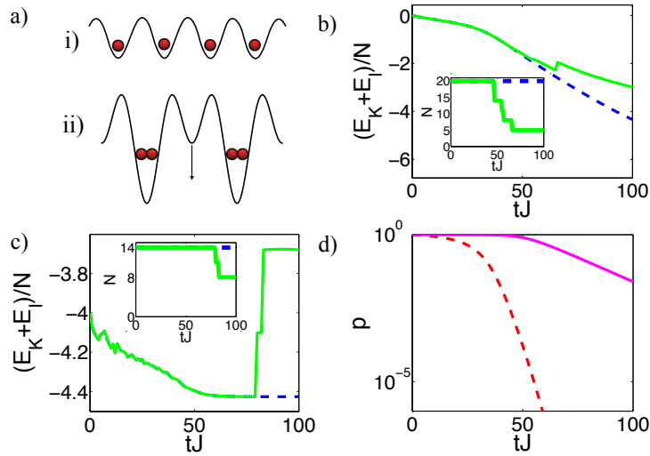
FIG. 25: Dynamics of adiabatic ramps into a dimer superfluid regime. (a) We begin with (i) a Mott insulator state (ramping U/J ), and (ii) a state with pre-prepared dimers in a superlattice (removing the superlattice). (b)-(c) The sum of kinetic ( E_K ) and interaction ( E_I ) energy and (inset) particle number as a function of time for two example trajectories, one with no loss events (dashed lines) and one with several loss events (solid lines). Here, (b) shows a ramp from U/J = 30 to U/J = -8 , with U(t) = \alpha J / (100 + 3tJ) + \gamma , with \alpha and \gamma ramp parameters, and (c) shows a ramp with a superlattice potential, \varepsilon_l = V_0 \cos(2\pi l/3) , where V_0 \approx 30J \exp(-0.1tJ) , adjusted so that V_0(tJ = 100) = 0 , with fixed U/J = -8 . In each case, \gamma_3 = 250J . For (b), we use 20 atoms on 20 lattice sites, for (c), 14 atoms on 23 lattice sites. (d) Plot showing the probability that no loss event has occurred after time t for the ramps in (b) (dashed line) and (c) (solid). Reprinted figure from A. J. Daley, J. M. Taylor, S. Diehl, M. Baranov, and P. Zoller, Phys. Rev. Lett 102 , 040402 (2009). Copyright 2009 by the American Physical Society.
