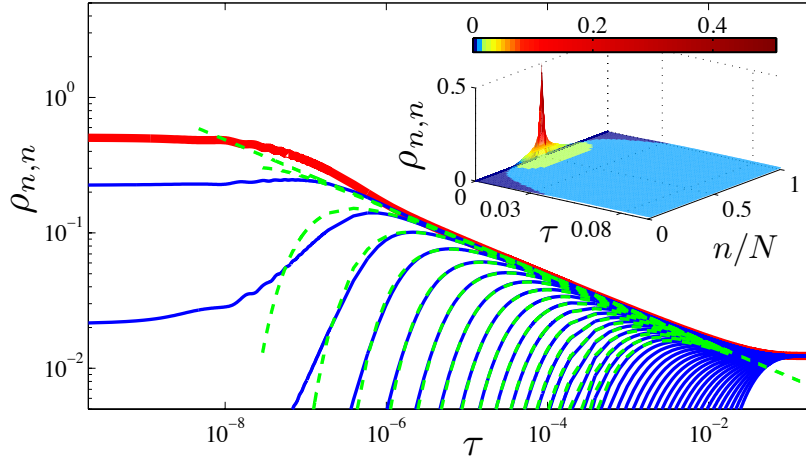
FIG. 17: Diagonal terms of the density matrix \rho_{n,n} , with \rho = \sum \rho_{n,m}|n\rangle\langle m| versus rescaled time \tau in log-log form: the exact solutions of Eq. (71) for n = 41 (top)...80(bottom) are represented by blue continuous lines; the element n = 40 (thick red line) is proportional to the probability of finding a balanced configuration P_b ; the corresponding diffusion density p(x = n/N, \tau) Eq. (5) of Ref. [82] up to n/N = 60 are shown in dashed green lines. Inset: 3D plot of the evolution. Parameters: U/J = 20 , \hbar\gamma/J = 1 , N = 80 and L = 2 . Reprinted figure with permission from D. Poletti, J.-S. Bernier, A. Georges, and C. Kollath, Phys. Rev. Lett 109 , 045302 (2012). Copyright 2012 by the American Physical Society.
