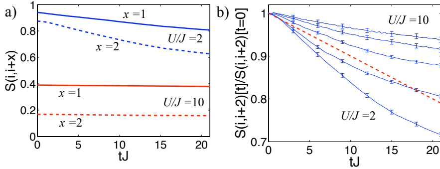
FIG. 16: Comparison of the decay of off-diagonal correlations in the single particle density matrix S(i, j) = \langle a_i^\dagger a_j \rangle as a function of time. These are computed from the master equation for the lowest band Eq. (71) with \gamma/J = 0.01 for 24 particles on a 24 site lattice by combining quantum trajectories methods with t-DMRG. (a) Comparison of the decay of off-diagonal elements \sum_i S(i, i+x) when U/J = 2 (superfluid regime, upper lines) and U/J = 10 (Mott Insulator regime, lower lines). In each case we show correlations at separation distances x = 1 (solid lines) and x = 2 (dashed lines), each of which are averaged over i . We see that the correlations for the Mott Insulator state at U/J = 10 are almost constant, whereas for U/J = 2 , the decay becomes more rapid than at initial times. (b) Comparison of S(i, i+2) averaged over i and normalized to the value at time t = 0 , |S(i, i+2)[t=0]| for U/J = 2, 4, 6, 8, 10 (seen here from bottom to top). The dashed line shows the corresponding result from perturbation theory. Each computation was averaged over 1000 trajectories, and error bars are shown in (b). For (a), the statistical errors fit inside the line thickness. Adapted from H. Pichler et al., Phys. Rev. A 82 , 063605 (2010) [81]. Copyright 2010 by the American Physical Society.
