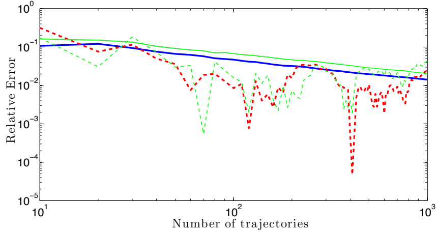
FIG. 6: Statistical errors in the quantum trajectories computation for hard-core bosons, taken from exact diagonalisation calculations with 5 particles on 10 lattice sites. Analogously to the two-level system case, we compare the statistical error estimate for our estimate of the energy E_{\text{bos}} (dark blue solid line) to the absolute error in the averaged value of E_{\text{bos}} when compared with the exactly computed value (dark red dashed line) at a time tJ = 8 . We also show the estimate of the error in a local correlation function \langle (a_5^\dagger a_6 + a_6^\dagger a_5) \rangle (light green solid line) compared with the discrepancy between this quantity and the exactly value (light green dashed line) at the same point in time. We show each of these values as a function of the number of trajectories over which we average, with all quantities plotted on a logarithmic scale. The statistical errors again decrease steadily \propto 1/\sqrt{N} for larger numbers, but the relative error in the local quantity remains larger than the global quantity.
