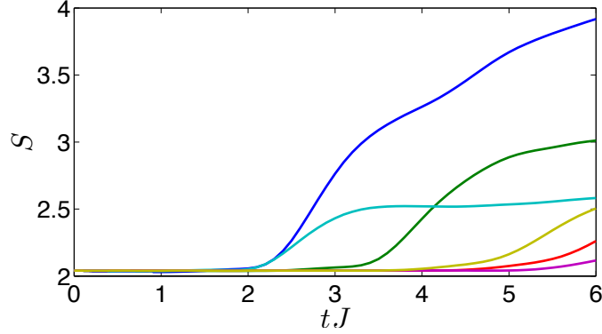
FIG. 11: Six example trajectories showing time-dependent DMRG simulations of the dynamics of 48 bosons on 48 lattice sites in a master equation with H = H_{BH} eq. (48), and jump operators c_m = a_m^\dagger a_m , and \gamma = 0.02J . Here we investigate the increase in the difficulty of the simulation as a function of time by plotting the von Neumann entropy across a splitting in the centre of the system (with 24 sites on each side). We see that there are different delays to the increase in S_{vN} , which depend on the timing of quantum jumps as well as their location with respect to the point of the bipartite splitting. All of these trajectories are exact calculations (t-DMRG truncation errors \epsilon_T lead to errors in S_{vN} that are smaller than the line thickness), with D = 256 .
