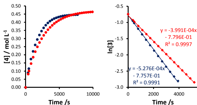
Figure 4. Kinetic data for the RCM of 3 ( 0.5 \text{ mol L}^{-1} , toluene- d_8 , 288 K with 250 ppm pre-catalyst), monitored by ^1\text{H} NMR spectroscopy: (a) concentration/time profiles; (b) first order treatment of kinetic data; SIPr in blue, SIPr OMe in red.
