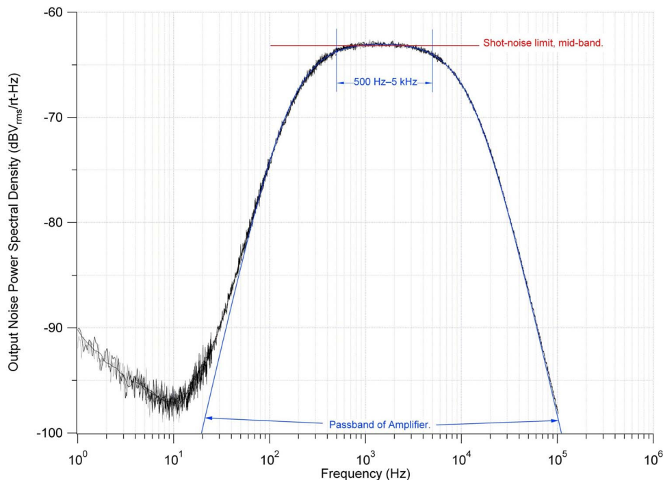
FIG. 5. Noise Power Spectral Density of the differential amplifier as a function of frequency, measured at the VM AC output of the amplifier. The fundamental mid-band shot noise limit is marked by the horizontal line in the figure, at -63.2\text{ dBV}_{\text{rms}}/\sqrt{\text{Hz}} . The theoretical amplifier Passband, as described by Eq. (2), is indicated by the blue line. Here, the fibre’s shadow fell over neither detector element, in order to avoid VM and other resonant peaks, and so the noise PSD is higher in this figure at 500\text{ Hz} , say, than when the shadow fell over the adjacent edge of both detector elements—as it must for proper VM detection. The reduction in noise PSD with the shadow present was approximately 0.8\text{ dB} , in fact. The noise reduction was due entirely to the lower levels of DC photocurrent, and so shot noise, in the two partially shaded PD elements. 7
