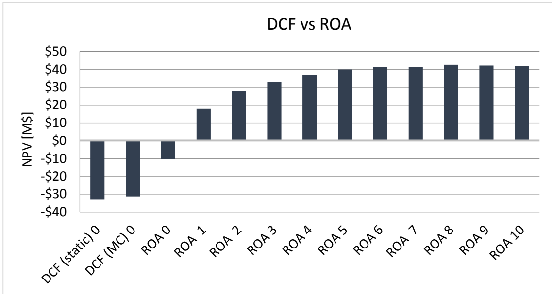
Figure 3. NPVs calculated with DCF methods and Real Options Approach at different years. Results for scenario 7 of desalination case.
