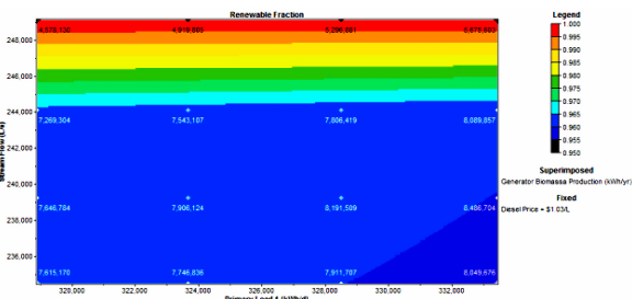
Figure 25 Effect of stream flow on renewable fraction
