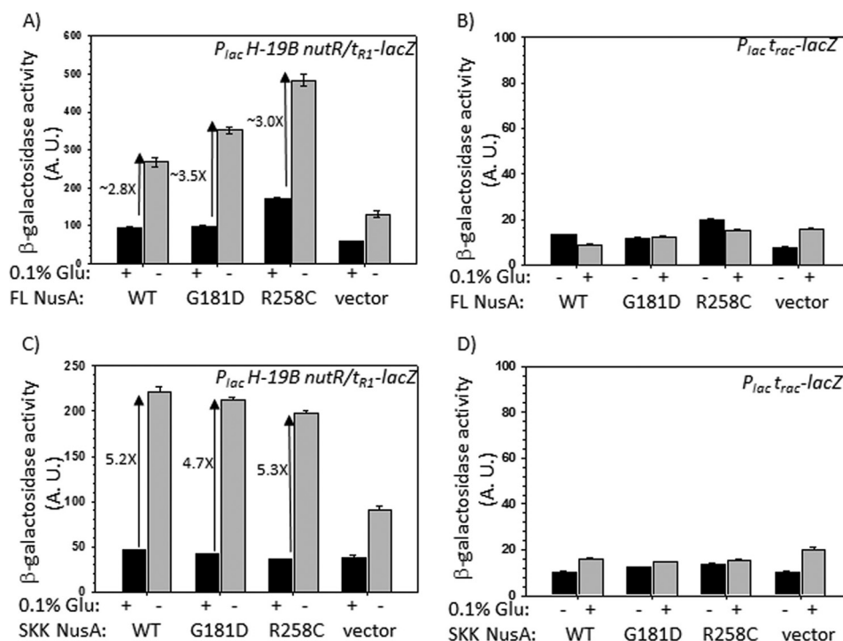
FIGURE 3. Effects of overexpression of full-length and SKK domain of NusA on the in vivo transcription. \beta -Galactosidase activities from the lacZ reporter fused downstream of Rho-dependent terminators, H-19B t_{R1} (A and C) and t_{rac} (B and D). The effects of overexpression of different derivatives of full-length (FL) NusA (A and B) and its SKK fragment (C and D) are shown. Concentrations of these two species were varied by adding (+) or omitting (-) 0.1% glucose ( Glu ) as they were expressed from the P_{BAD} promoter. In vivo levels of full-length NusA and SKK fragments were verified by Western blotting (data not shown). Because the in vivo levels of different NusA derivatives were similar (~3-fold enhancement upon induction), we did not attempt to normalize the \beta -galactosidase activities. S.D. values (error bars) were obtained from five independent measurements. vector , empty plasmid without the nusA . A.U., arbitrary units.
