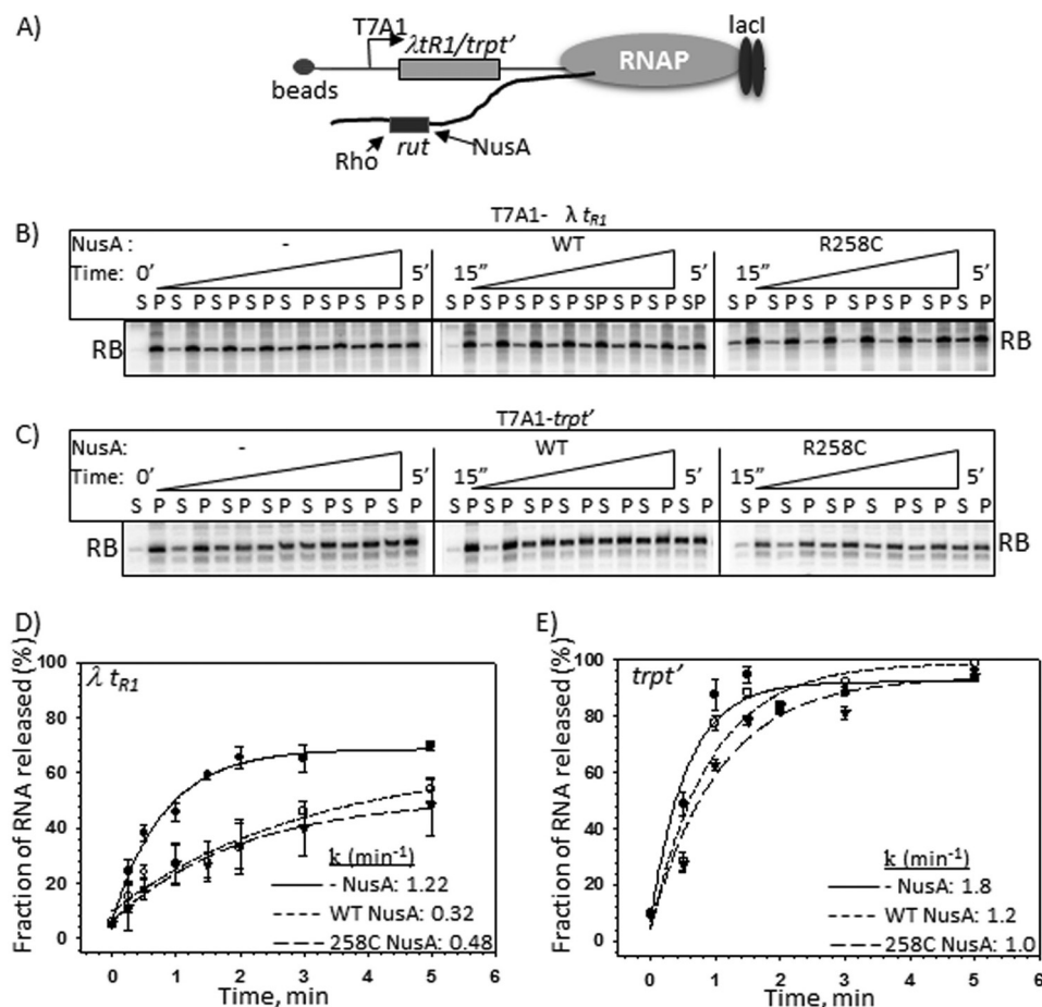
FIGURE 5. Assays to show direct NusA-Rho competition for the overlapping nut and rut sites. A, schematic showing the configuration of the stalled ECs at a Lacl roadblock (RB) downstream of either \lambda tr_{R1} or trpt' terminators. DNA templates were immobilized to magnetic beads via a streptavidin-biotin linkage. This immobilization enables us to measure the released RNA in the solution. Rut sites of each of the terminators are indicated. Autoradiograms show the time courses of RNA release from the ECs stalled downstream of either \lambda tr_{R1} (B) or trpt' (C) terminators. These time courses were obtained either in the absence of NusA or in the presence of WT or R258C NusA. Inverted triangles denote the increasing time as indicated. S and P, one-half of the supernatant and one-half of the supernatant plus pellet fractions, respectively. D and E, plots of fractions of released RNA obtained in B and C, respectively, against time. The indicated rates of RNA release ( k ) for each curve were calculated from the exponential fitting of the curves. The fraction of released RNA was estimated from the expression, [2S]/([S] + [S + P]) . S.D. values (error bars) were calculated from three independent measurements.
