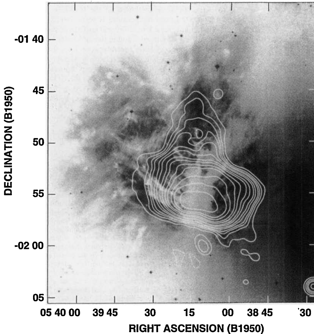
Figure 1. Contour representation of the 330-MHz image of NGC 2024 made with a beam of FWHM 65.1 \times 64.6 arcsec 2 at a position angle (PA) of 61^\circ 2 . Contours are at 10 mJy beam -1 \times (-2, 2, 4, 6, 8, 12, 16, 24, 32, 48, 64, 96, 128, 192) . An optical image of NGC 2024 is shown in grey-scales.
