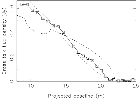
Figure 5. As the projected baseline between two antennas that are in a shadowed configuration decreases, the observed cross-talk amplitude (shown as a continuous line joining the box symbols) is compared with the area of the back antenna that is geometrically shadowed (dotted line) and the length of the rim of the front antenna that appears projected on the back antenna aperture (dashed line). The observed cross-talk amplitudes displayed are at 4800 MHz; the vertical scales for the rim length and shadowing area are arbitrary.
