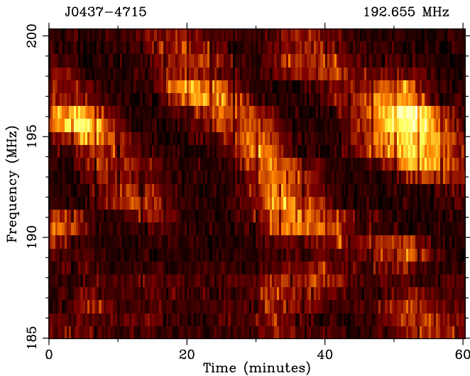
Figure 2. Dynamic spectrum of the pulse intensity from the MWA observations of PSR J0437–4715 over a time duration of 1 hr and a bandwidth of 15.36 MHz centered at 192.655 MHz. The time and frequency resolutions in this plot are 20 s (i.e., one sub-integration) and 0.64 MHz, respectively.
