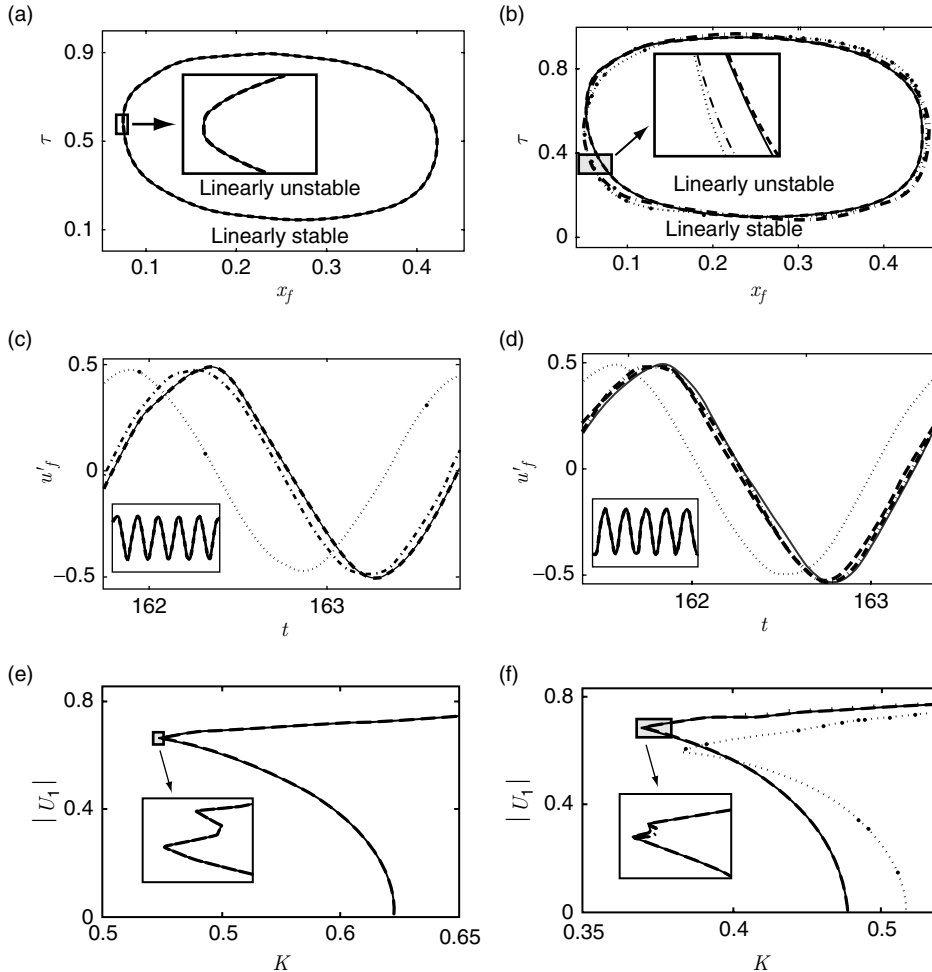
Figure 2: Modal convergence of linear stability boundary between x_f and \tau with (a) c_1 = 0.1 , c_2 = 0.06 and K = 0.8 (b) c_1 = 0.05 , c_2 = 0.06 and K = 0.8 . In this Figure, ..... N = 1 , -.-.- N = 2 , - - - N = 9 and — N = 10 . Comparison of limit cycle amplitude from time evolutions with different number of acoustic Galerkin modes ( N ) with x_f = 0.3 and \tau = 0.2 (c) for case shown in 2(a) and (d) for case shown in 2(b). Comparison of bifurcation plots for variation of non-dimensional heater power ( K ) with different number of acoustic Galerkin modes ( N ) (e) for system in 2(a) (f) system in 2(b). Grey areas are enlarged in inset figures to show convergence with increase in number of modes.
