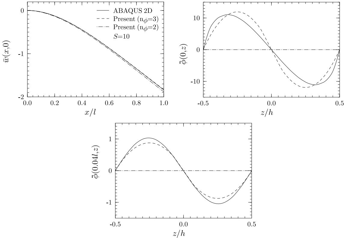
Figure 10. Deflection profile and distribution of \bar{\phi} for shear pointer beam (d) under pressure load 2.
