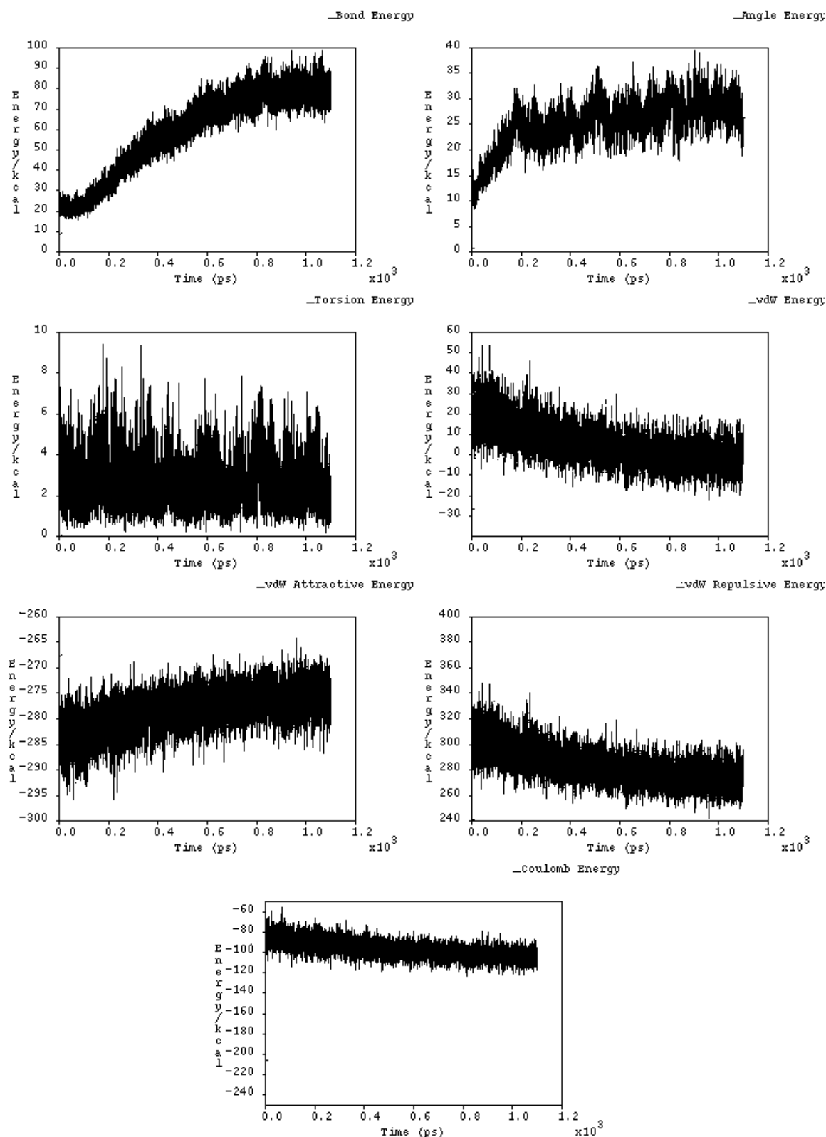
Figure 3. Variations of bond energy, angle energy, torsion energy, vdw energy, vdw attractive energy, vdw repulsive energy and Coulomb energy with time during MD simulation.
