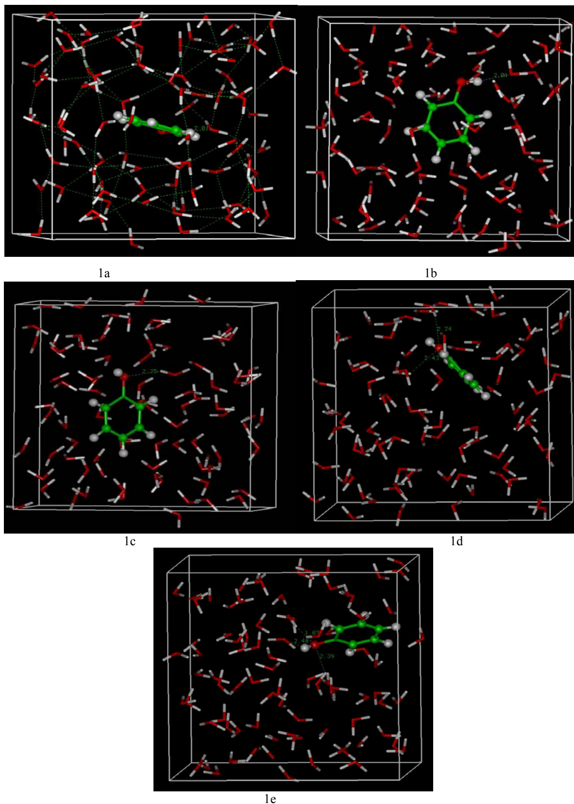
Figure 1. (a) Molecular structure of phenol–water cluster. (b) Molecular plane of the phenol with hydrogen bonded network of whole system. (c) Molecular structures obtained after 400 ps. (d) Molecular structures obtained after 600 ps. (e) Molecular structures obtained after 1000 ps.
