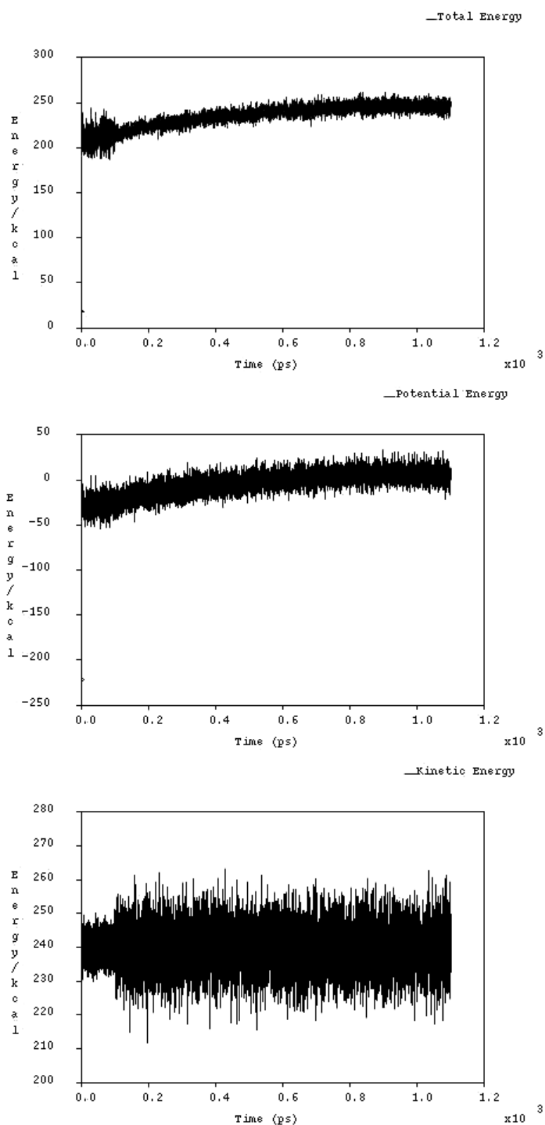
Figure 2. The variation of total energy, potential energy and kinetic energy during molecular dynamics.
