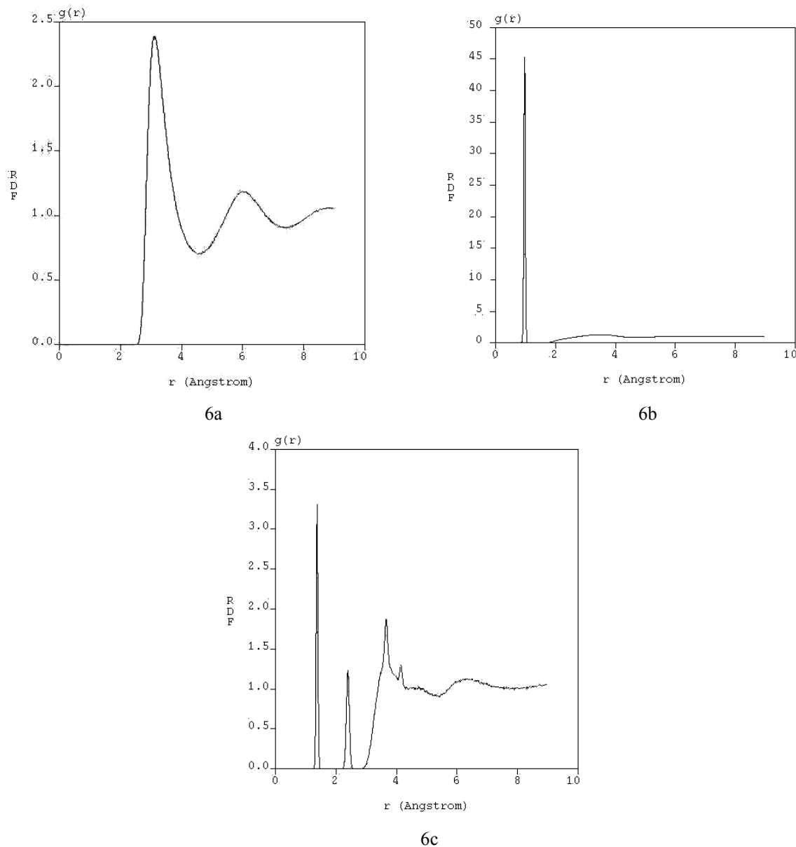
Figure 6. (a) Radial distribution function (RDF) O–O atoms. (b) RDF for O–H atoms. (c) RDF for C–O atoms.
