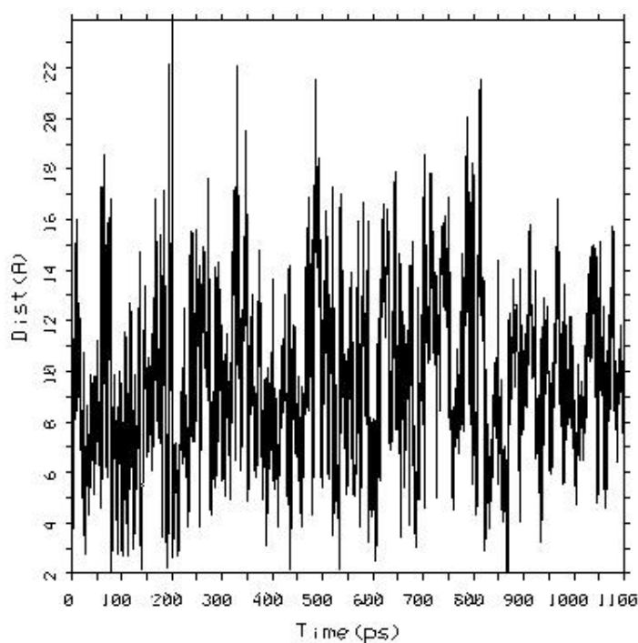
Figure 4. MD trajectories of the hydrogen bond distance between phenol and water molecule.
