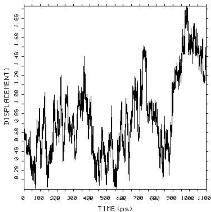
Figure 5. Displacement of phenol–water cluster during 1 ns.
