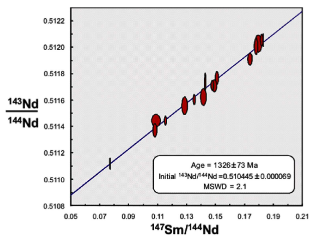
Fig. 3: Nd isotopic analyses (measured by LA-MC-ICP-MS) and isochron age of the apatite grains from the Racherla syenite (see Chalapathi Rao et al. , 2012d)
