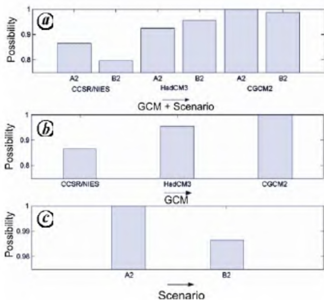
Figure 4. Possibility values assigned to GCMs and scenarios (Mujumdar and Ghosh) 7 .
