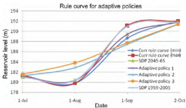
Figure 8. Reservoir operation under CGCM2 A1B scenario: current rule curve versus mean elevations obtained for adaptive policies.
