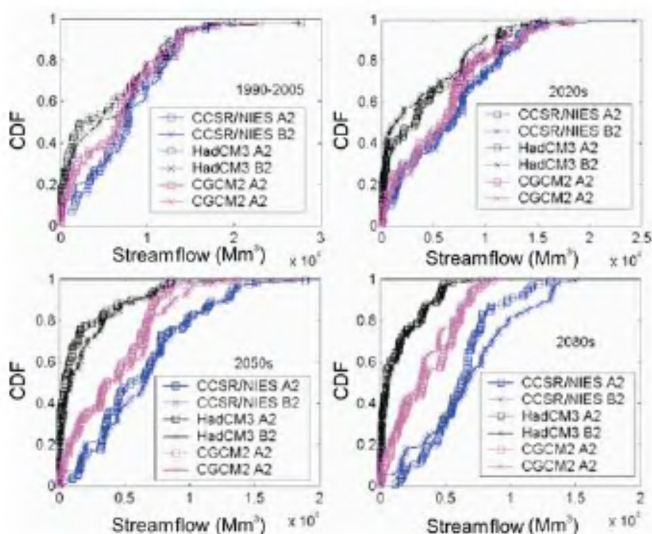
Figure 3. Predicted streamflow with different GCMs and scenarios (Mujumdar and Ghosh) 7 .
