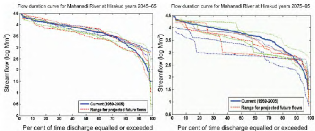
Figure 6. Range of projected future flow duration curves for monsoon inflows at Hirakud for two time slices, 2045-65 and 2075-95.
