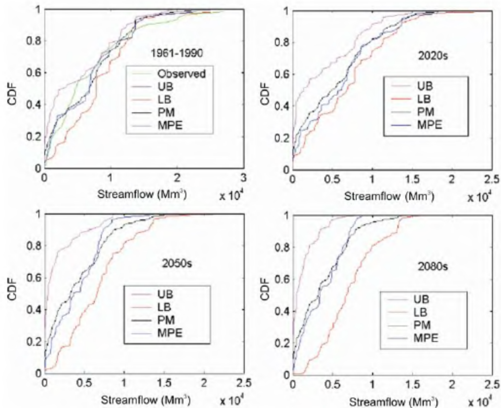
Figure 5. Upper bound (UB), lower bound (LB) and possibilistic mean CDF. PM, possibilistic mean; MPE, most possible experiment.
