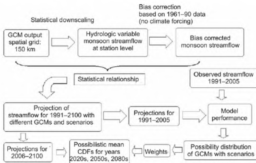
Figure 2. Possibilistic approach for modelling GCM and scenario uncertainty (Mujumdar and Ghosh 7 ).
