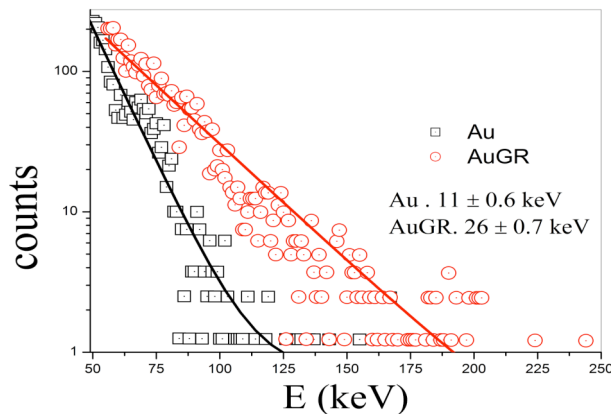
Figure 2: Bremsstrahlung spectra obtained from AuGR and polished Au surface. The “hot” electron temperature in the both the cases are found to be 26 \pm 0.7 keV and 11 \pm 0.6 keV respectively.
