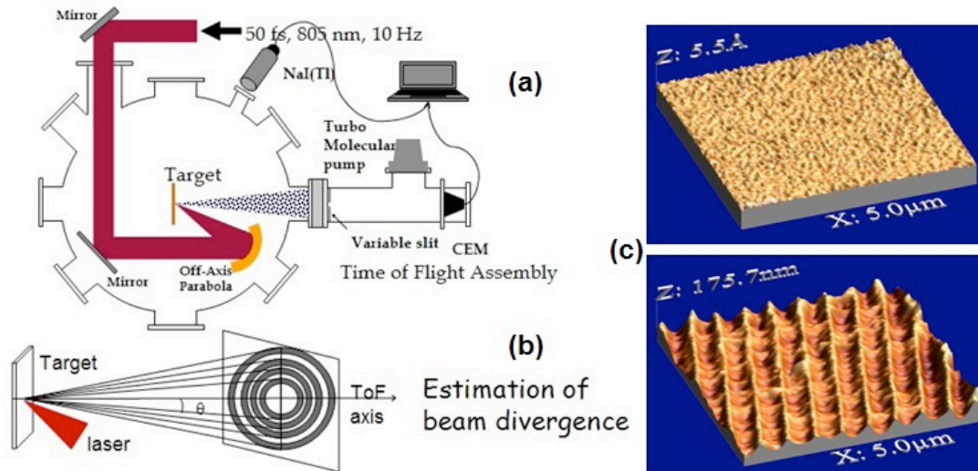
Figure 1: Schematic diagram of the (a) experimental set up (b) annular FCs (AnFC). (c) AFM images of the polished gold surface (Au) and sub- \lambda grating (AuGR) used in the experiments.
