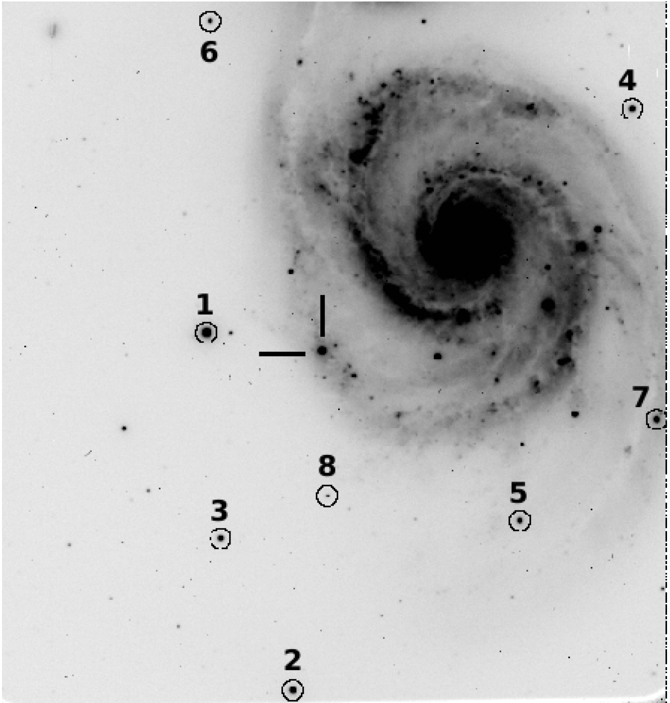
Figure 1. Identification chart for SN 2011dh. The stars used as local standards are marked with numbers 1–8. North is up and east to the left. The field of view is 10 \times 10 arcmin 2 .
