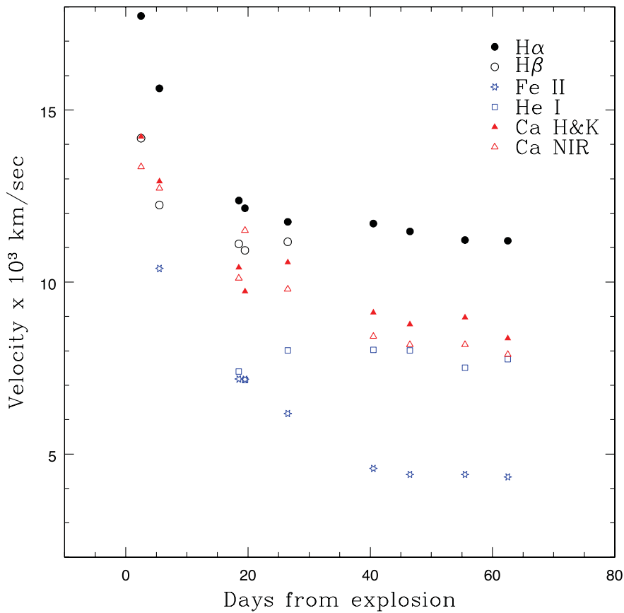
Figure 17. Evolution of the expansion velocity of supernova ejecta measured using different species.
