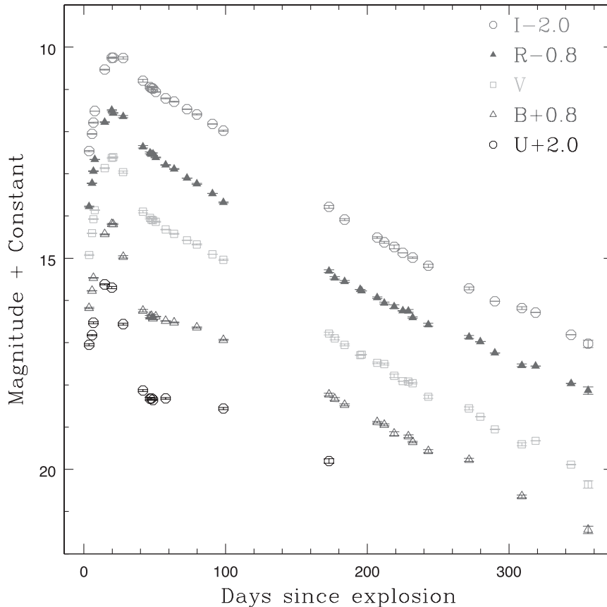
Figure 2. UBVR light curves of SN 2011dh. The light curves have been shifted by the amount indicated in the legend.
