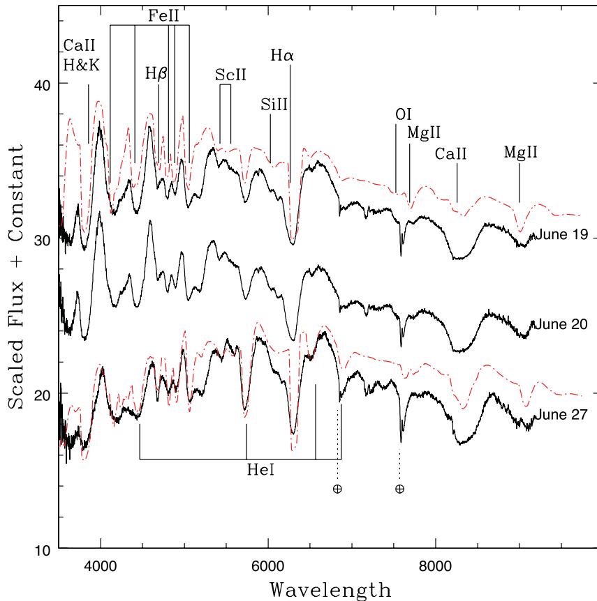
Figure 9. Spectral evolution of SN 2011dh during \sim 20 to \sim 27 d after explosion. The observed spectra (black) have been plotted with the synthetic spectra (red, dash-dotted) created using SYN++.
