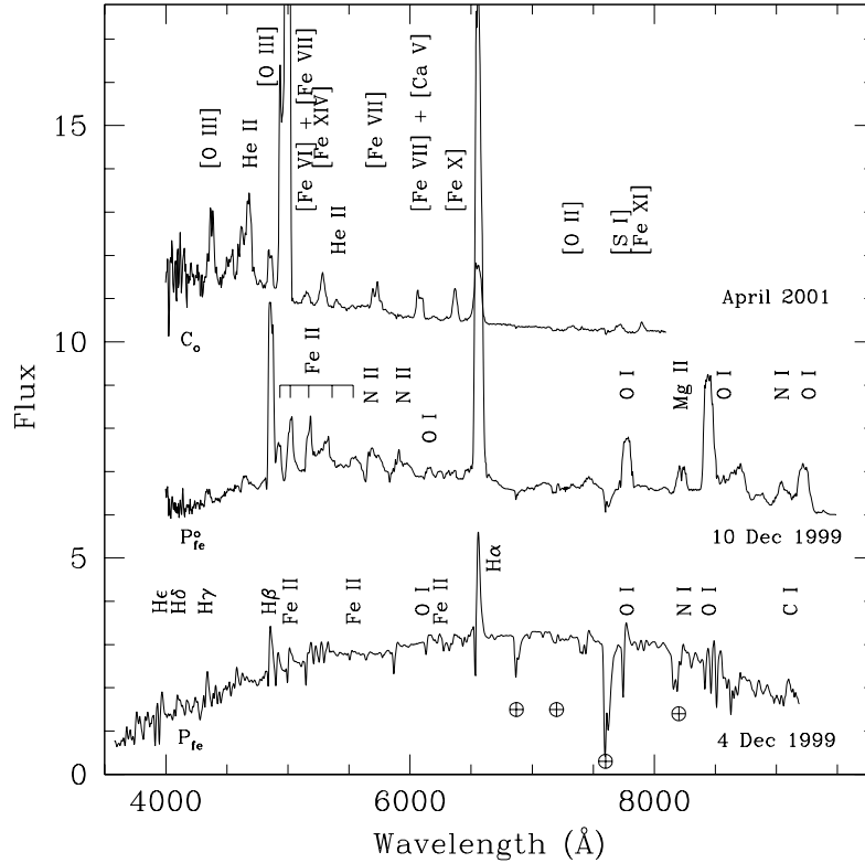
Figure 2. The evolutionary sequence of nova V1494 Aql showing the change from a permitted to coronal spectrum as labelled on the left side of each spectrum. Dates of observations are labelled on the right side of each spectrum. Prominent lines are labelled.
