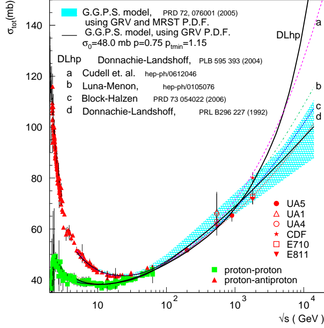
Fig. 3: Results from our total cross-section model (for different parton densities) compared with data [11] and with other models [12].
