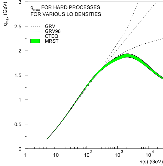
Fig. 2: Results for q_{max} using different input parton densities with p_{tmin} = 1.15 GeV.
