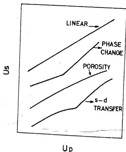
Figure 1. Schematic U_s - U_p curves.
