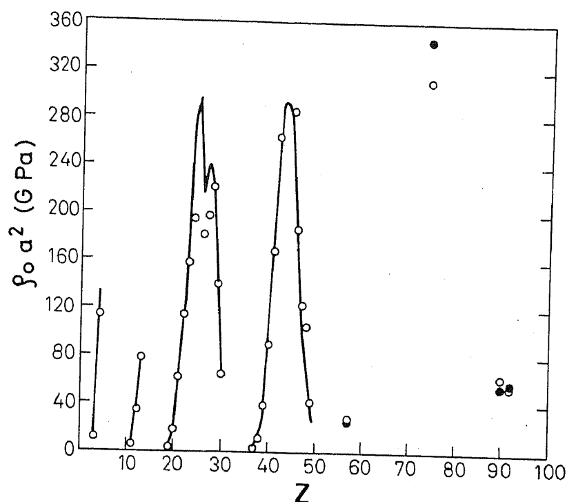
Figure 3. Shock bulk modulus of elements versus Z .
