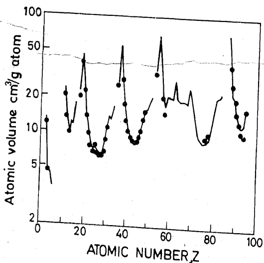
Figure 2. Zero pressure atomic volumes of elements versus the atomic number. The experimental values lie along the quasi continuous lines. Those calculated by band theory are represented by points.
