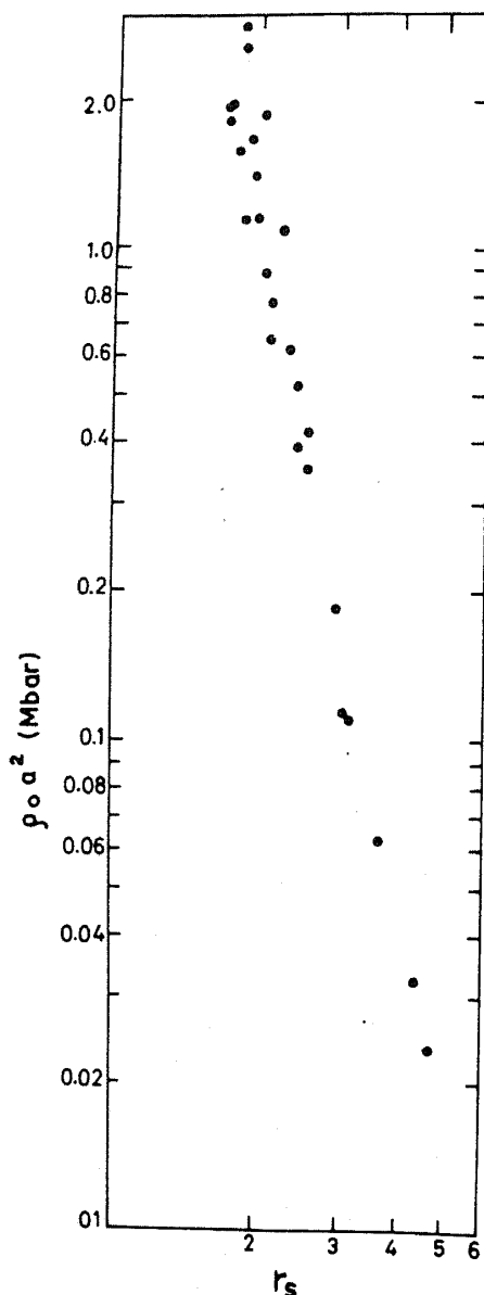
Figure 4. Shock bulk modulus ( \rho_0 a^2 ) versus the electron density parameter r_s for elements.
