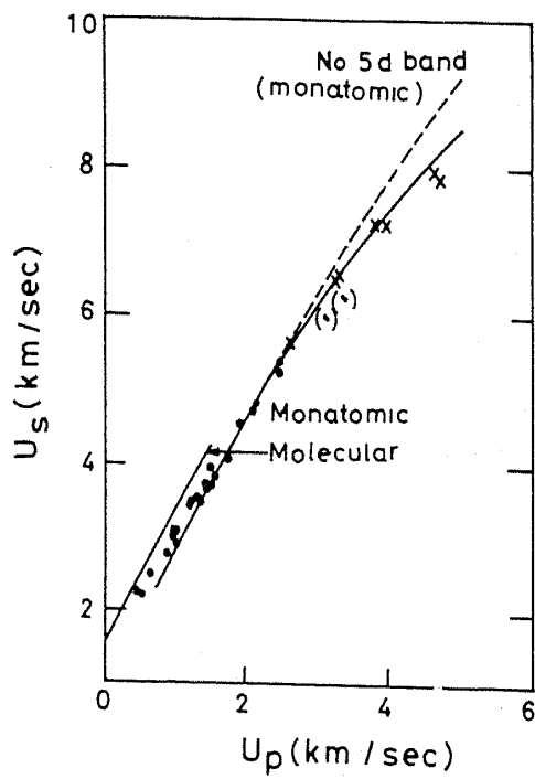
Figure 11. U_s - U_p curve for iodine (McMahan et al 1977).
