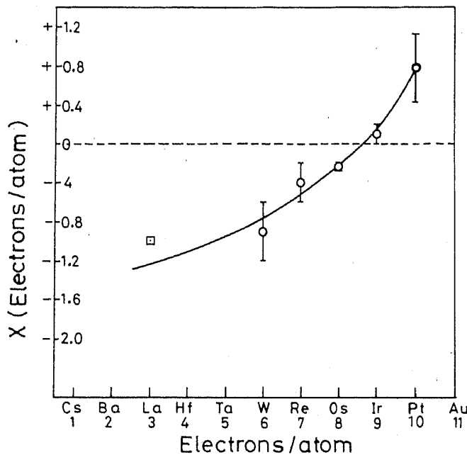
Figure 8. The available experimental values of s \rightleftharpoons d electron transfer parameter for the 5d transition series (Svechkarev and Panfilov 1974).
