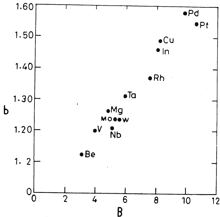
Figure 5. b versus the repulsive parameter B .
