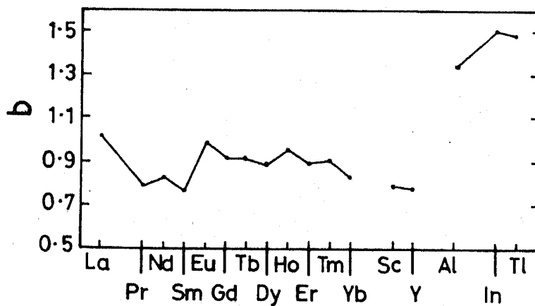
Figure 6. Experimental b values for trivalent elements.
