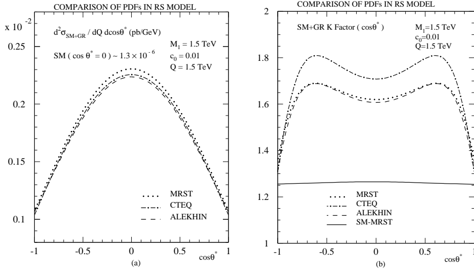
Figure 1. (a) In the region of first RS resonance, the double differential with respect to invariant mass and angular distribution of the lepton is plotted for various PDFs at LHC. (b) The corresponding K-factor for various PDFs.
