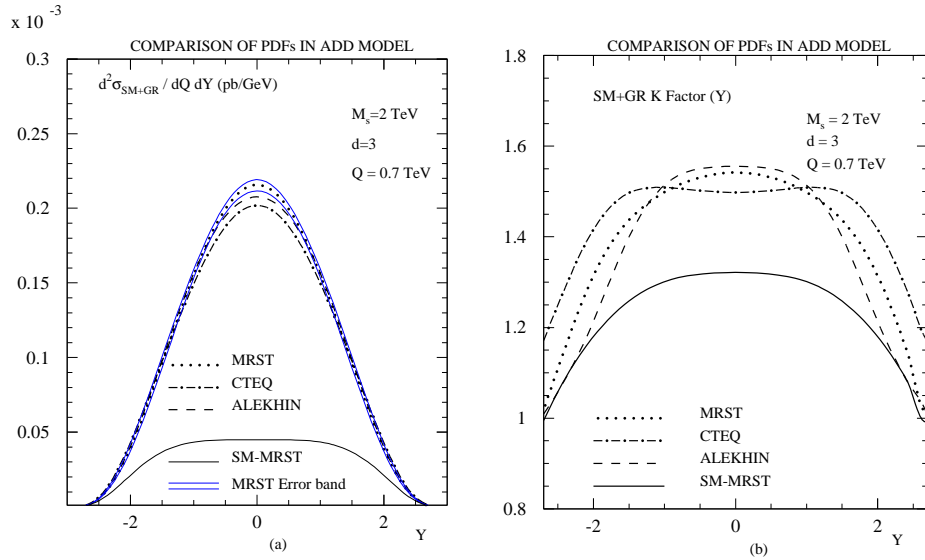
Figure 2. The comparison plots for the various PDF sets for Q = 0.7 \text{ TeV} at LHC. (a) The double differential cross-section with respect to invariant mass and rapidity as a function of rapidity. The thin line band gives the range of experimental error on the MRST PDF. (b) The corresponding K-factor as a function of rapidity.
