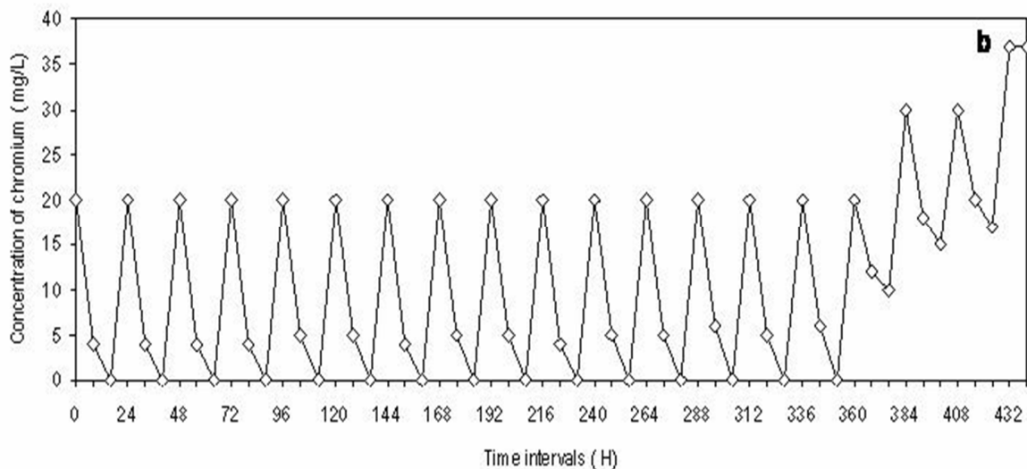
Figure 4b: Reduction of Cr (VI) in continuous (repeated) addition of Cr (VI) at 20 mg/L at 24 h by the marine B.licheniformis .
