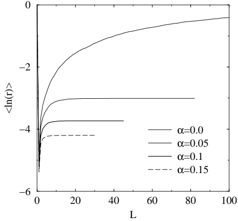
FIG. 6. Average of logarithm of reflection coefficient versus sample length for a fixed value of disorder W = 1.0 and different values of absorption \alpha indicated in the figure.
