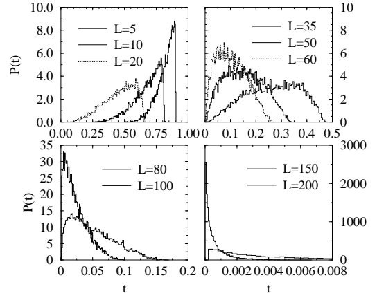
FIG. 4. Distribution of transmission coefficient t from a disordered absorptive system with W = 1.0 and \alpha = 0.01 at different lengths L .
