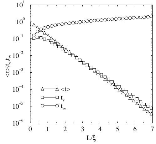
FIG. 3. Average transmission coefficient \langle t \rangle , variance of t ( t_v ) and relative variance of t ( t_{rv} ) as a function of L/\xi for fixed disorder W = 1.0 and absorption \alpha = 0.01 .
